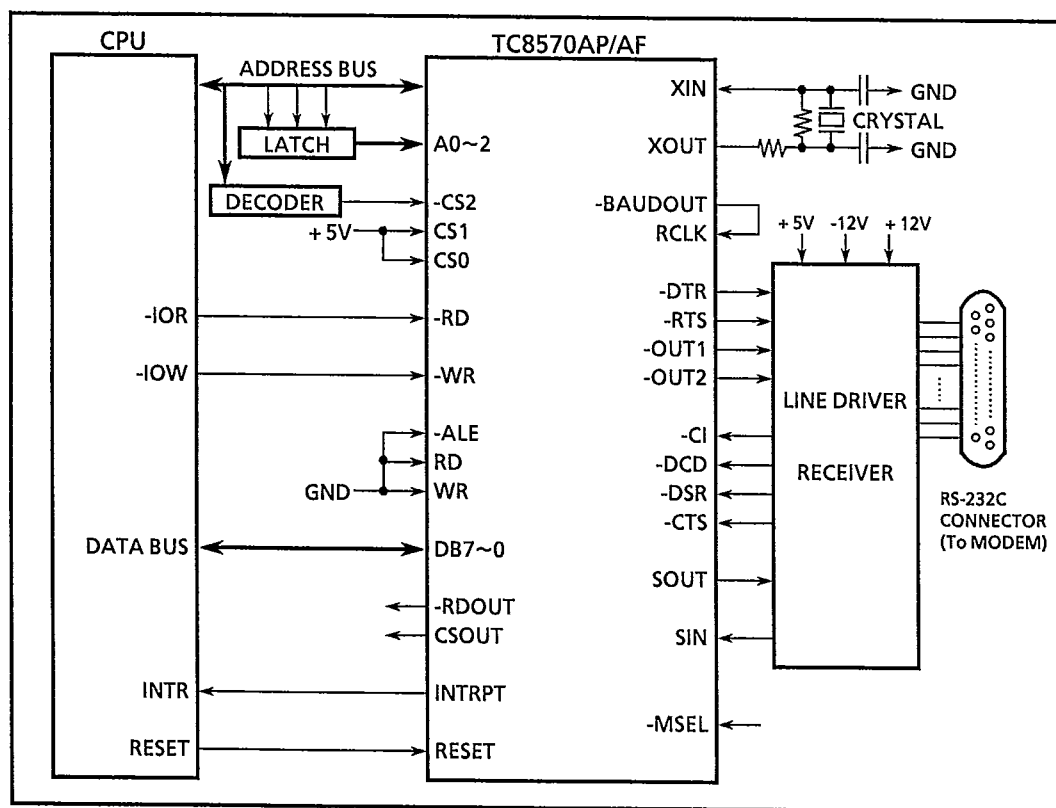
FIG.3.2 SYSTEM CONFIGURATION
