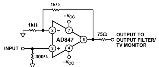
Figure 95. Recommended Output DAC Buffer
