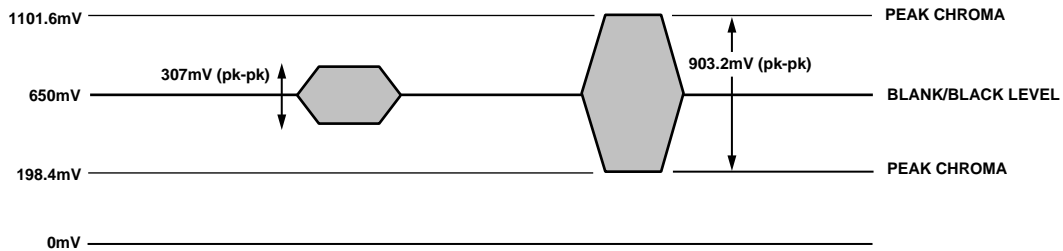
Figure 80. NTSC Chroma Video Levels
