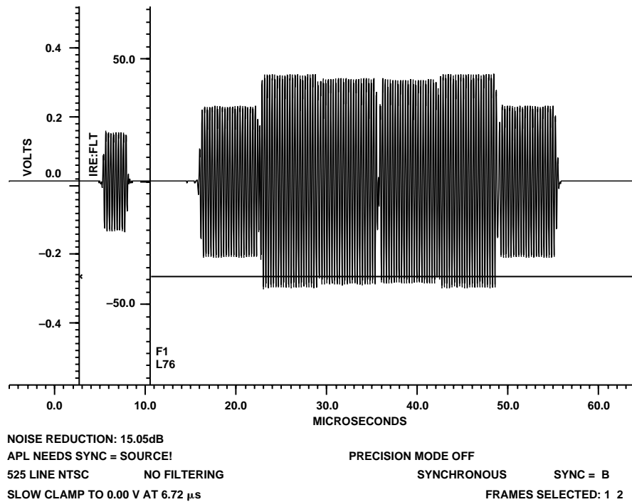
Figure 101. 100%/75% NTSC Color Bars Chrominance
