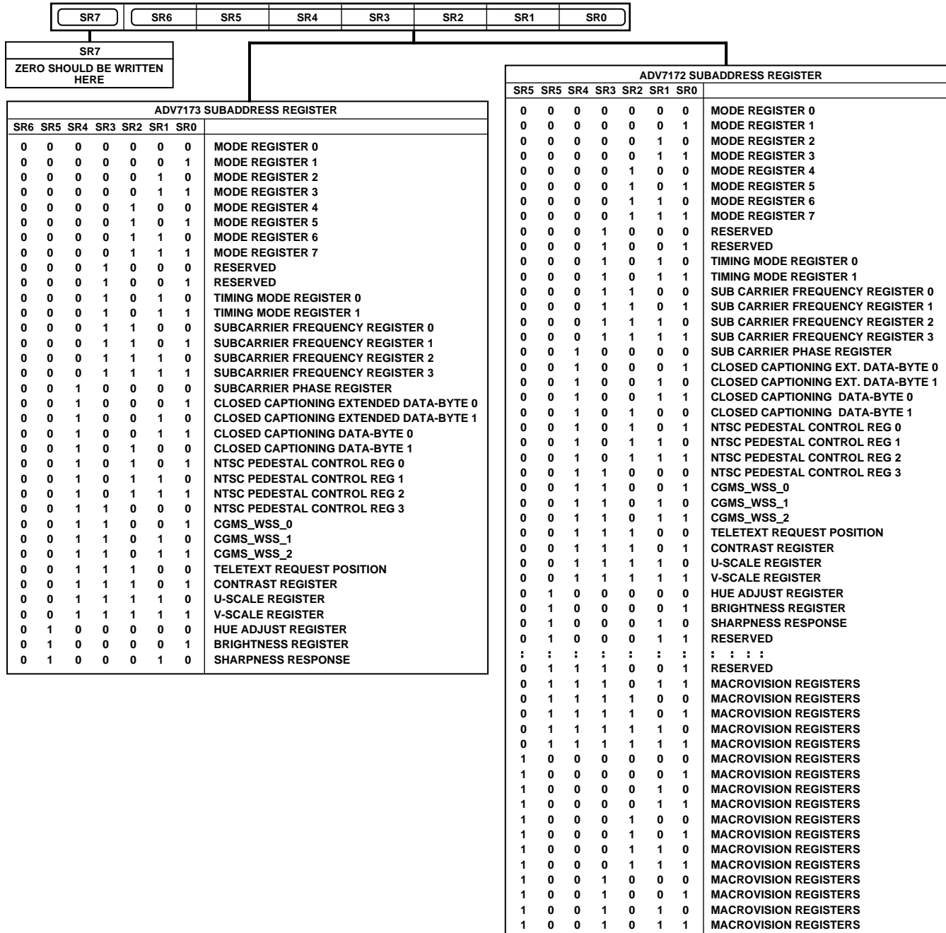
Figure 43. Subaddress Register
