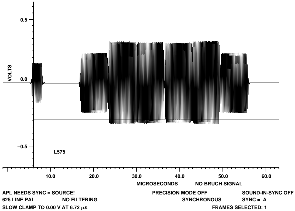
Figure 98. 100%/75% PAL Color Bars Chrominance
