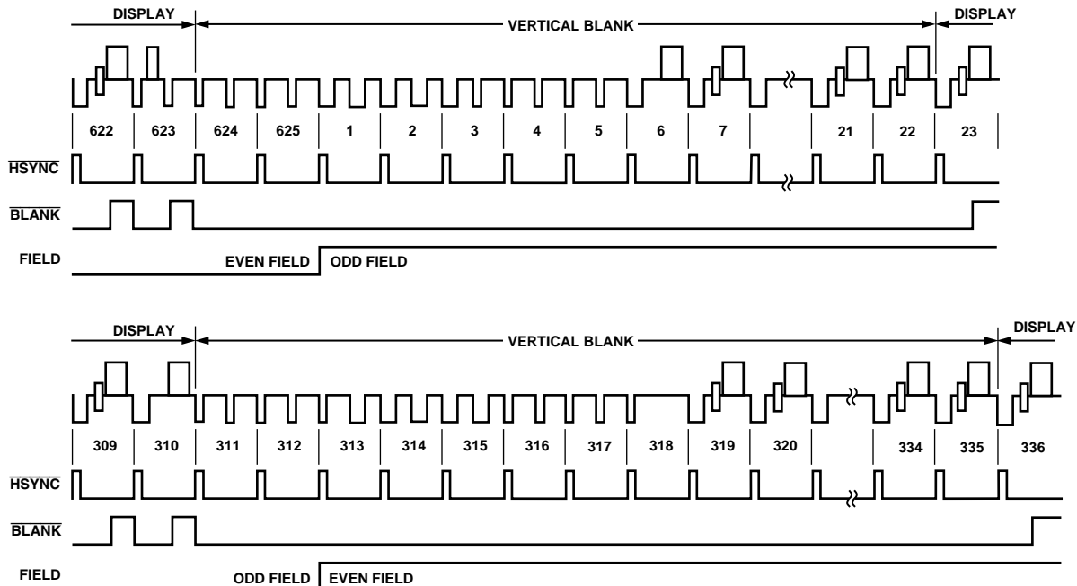
Figure 35. Timing Mode 3 (PAL)
