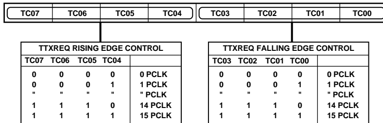
Figure 59. Teletext Control Register
