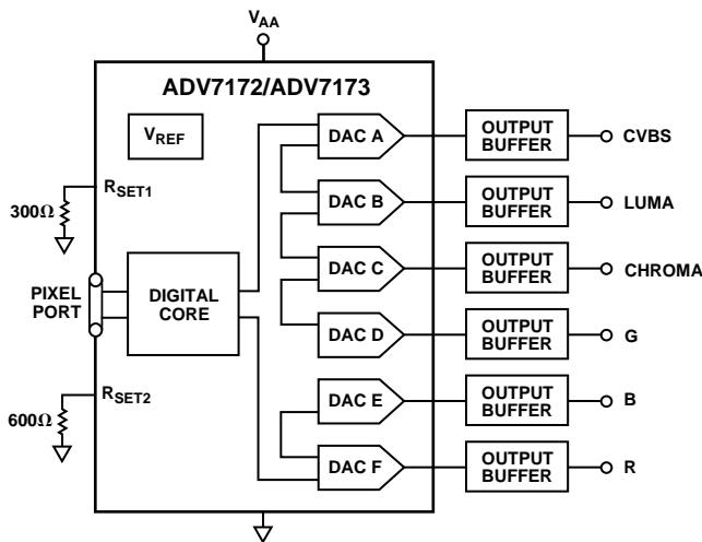
Figure 94. Output DAC Buffering Configuration
