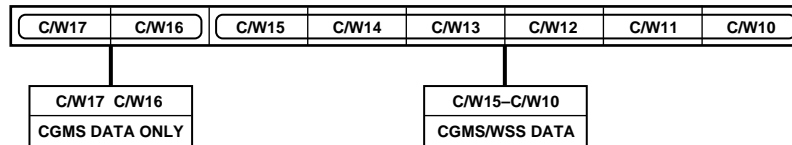
Figure 61. CGMS_WSS Register 1
