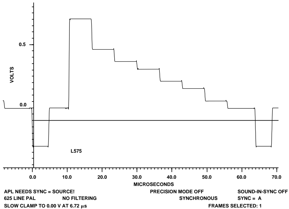
Figure 97. 100%/75% PAL Color Bars Luminance
