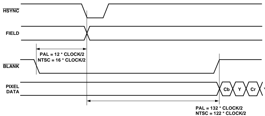
Figure 29. Timing Mode 1 Odd/Even Field Transitions Master/Slave
