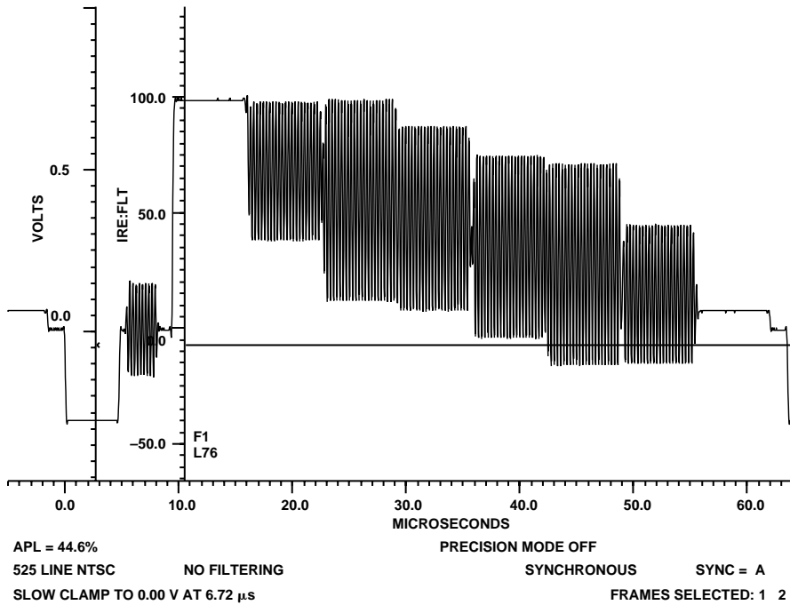
Figure 99. 100%/75% NTSC Color Bars
