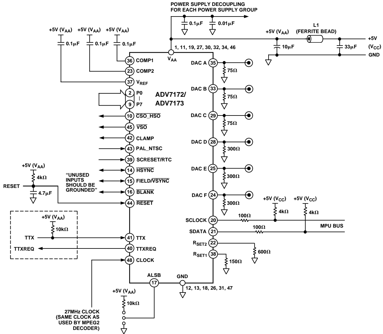
Figure 68. Recommended Analog Circuit Layout
