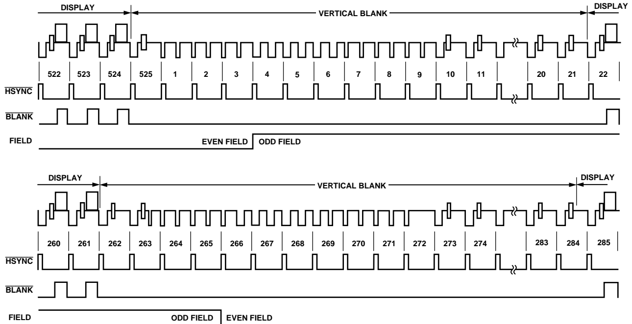
Figure 34. Timing Mode 3 (NTSC)
