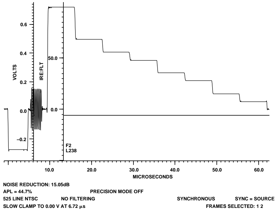
Figure 100. NTSC Color Bars Luminance
