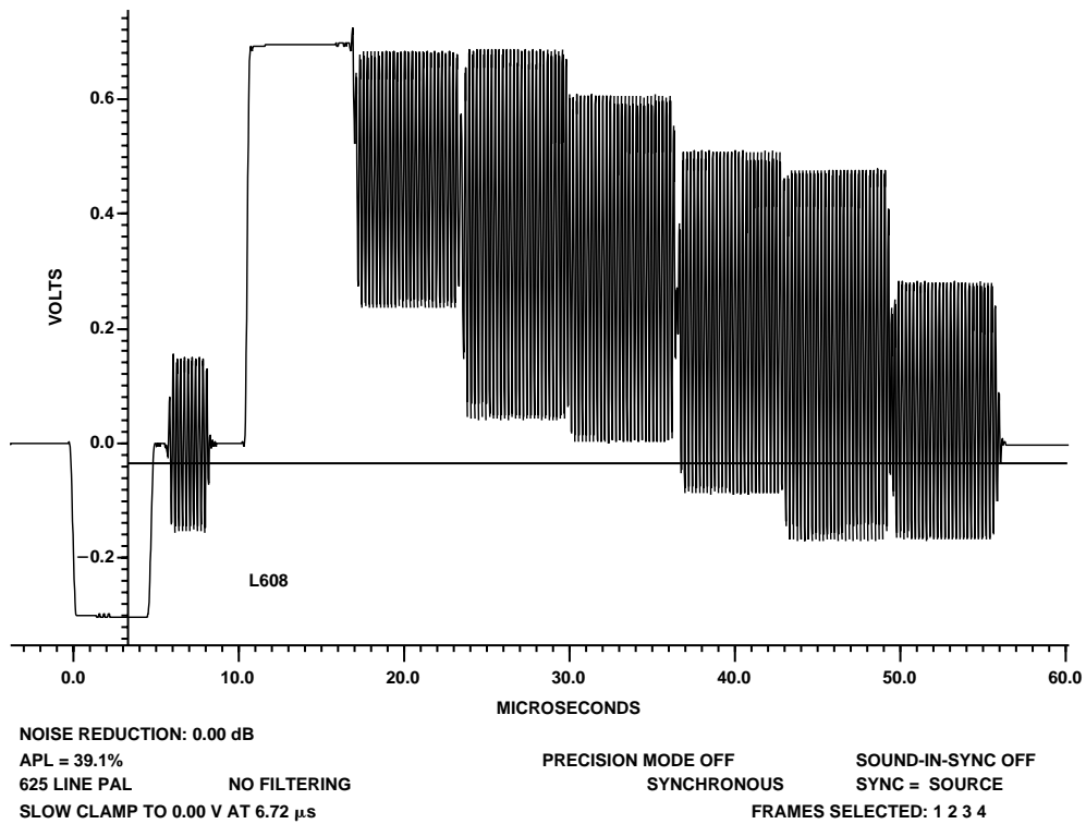
Figure 96. 100%/75% PAL Color Bars
