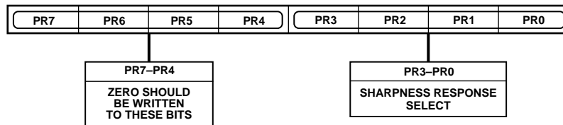
Figure 67. Sharpness Response Register
