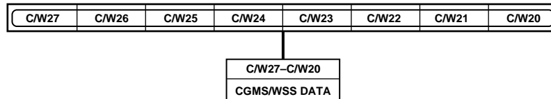
Figure 62. CGMS_WSS Register 2
