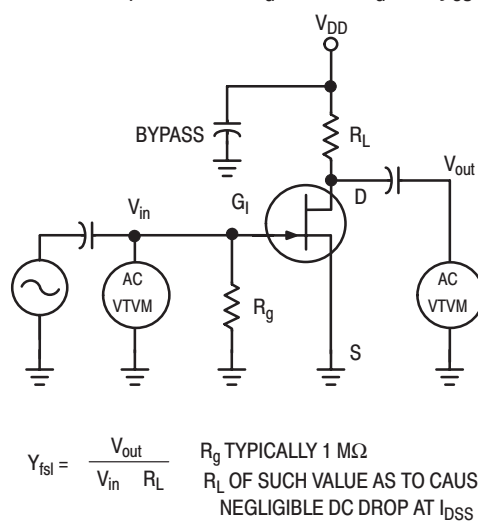
Figure 13. Typical y_{fs} Test Circuit
