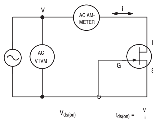
Figure 20. Circuit for Measuring JFET Channel Resistance
