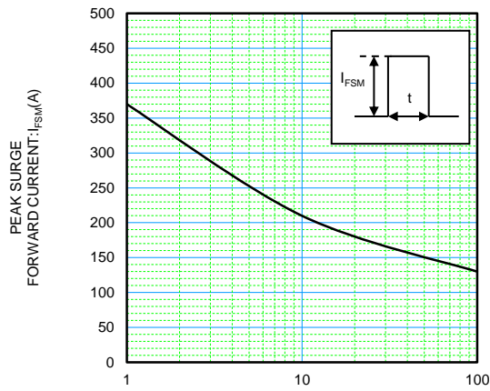
I_{FSM} -t CHARACTERISTICS
