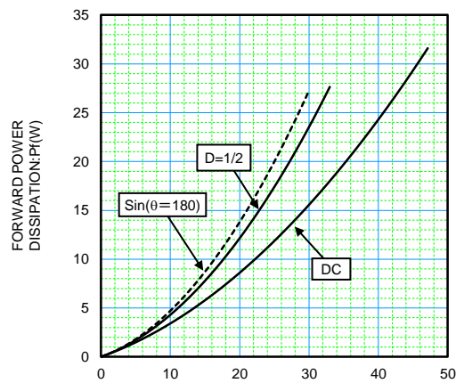
Io-Pf CHARACTERISTICS
