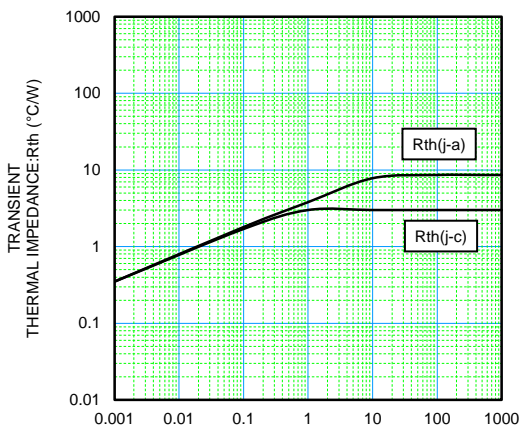
Rth-t CHARACTERISTICS
