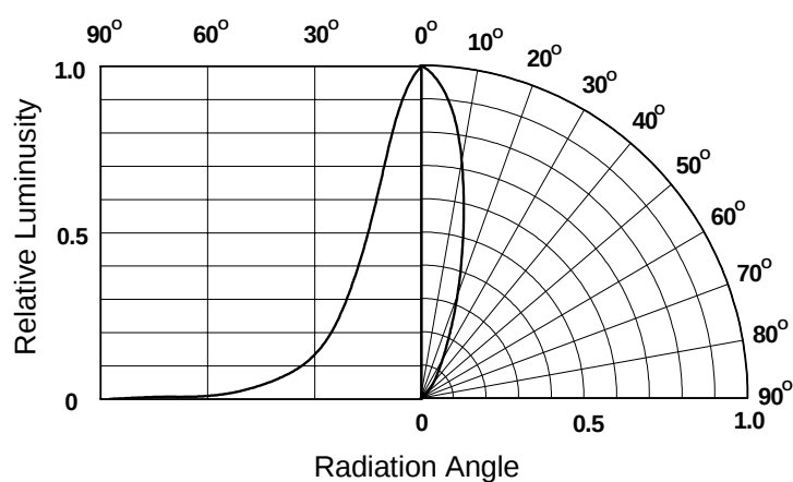
Radiation Characteristics
