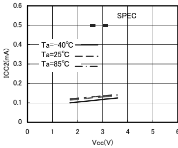
Fig.13 Current consumption at READ operation Icc2 (fsci=100kHz)
