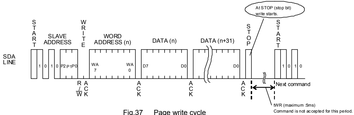
Fig.37 Page write cycle
