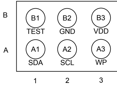
Fig.3 BU99901GUZ-W(bottom view)
