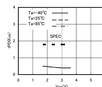
Fig.24 Data output delay time tPD0
