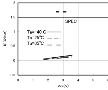
Fig.11 Current consumption at READ operation Icc2 (fsci=400kHz)
