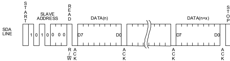
Fig.40 Sequential read cycle (in the case of current read cycle)
