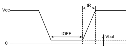
Fig.51 Rise waveform diagram
