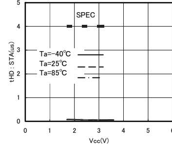
Fig.18 Start Condition Hold Time tHD : STA
