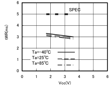
Fig.27 Internal writing cycle time tWR
