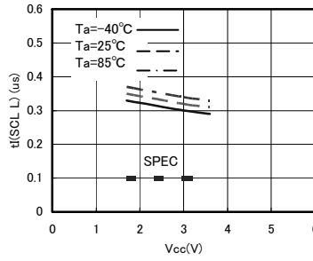
Fig.29 Noise reduction effect time t(SCL L)
