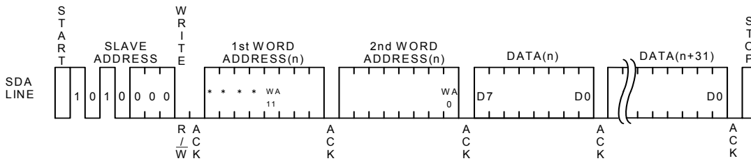
Fig.36 Page write cycle
