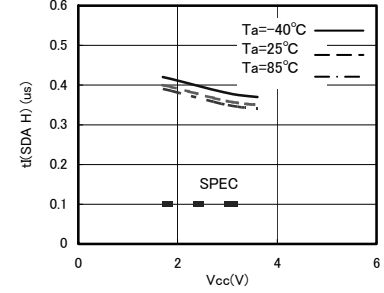
Fig.30 Noise reduction effect time t(SDA H)
