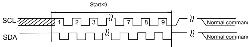
Fig.41-(c) START x 9 + command input
