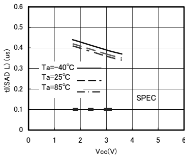
Fig.31 Noise reduction effect time t(SDA L)
