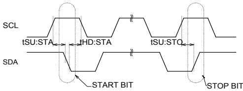
Fig.1-(b) Start - stop bit
