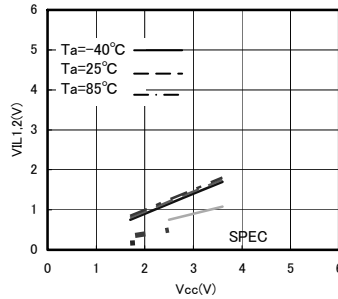
Fig.5 'L' input voltage V_{IL} (SCL,SDA,WP)
