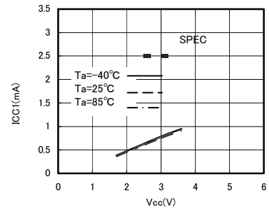
Fig.12 Current consumption at WRITE operation Icc1 (fsci=100kHz)
