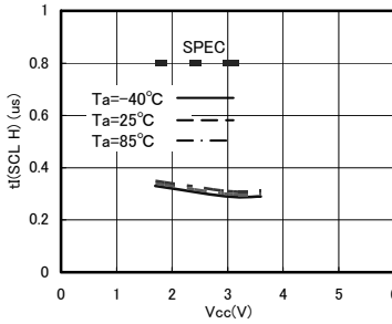
Fig.28 Noise reduction effect time t(SCL H)
