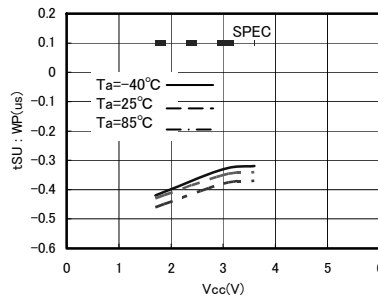
Fig.32 WP setup time tSU : WP
