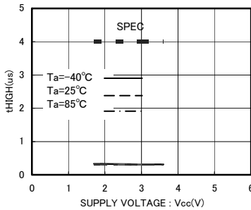
Fig.16 Data clock High Period tHIGH
