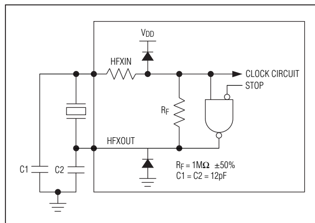
Figure 9. On-Chip Oscillator
