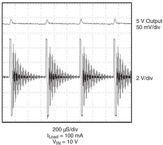
Pulse-Skipping Waveforms
