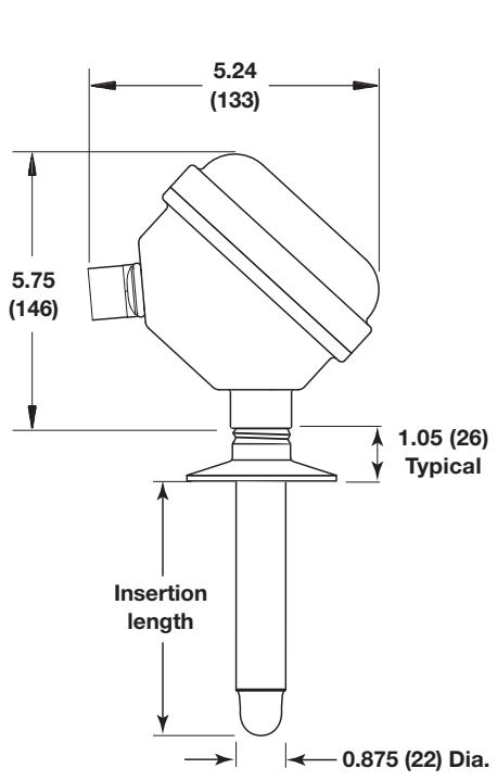
Model TD2 with Hygienic Housing Tri-Clamp® Connection
