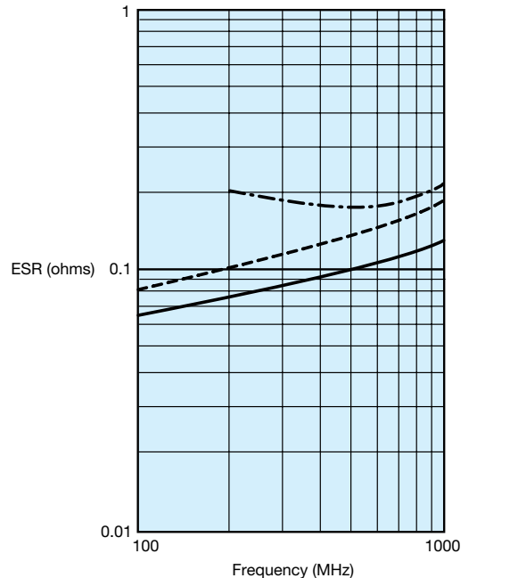
TYPICAL ESR vs. FREQUENCY AQ11/12 MIL-PRF-55681E - BP STANDARD - A
