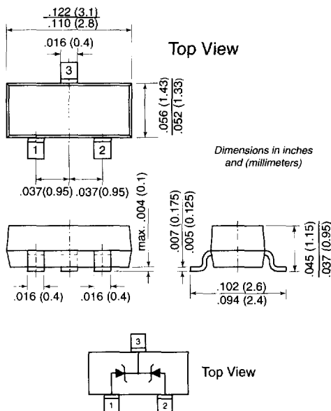
TO-236AB (SOT-23)
