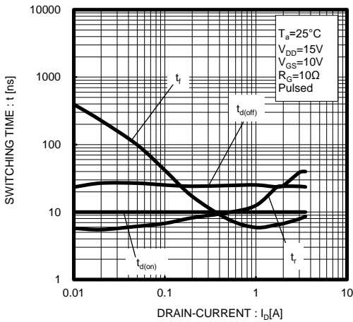
Fig.11 Switching Characteristics
