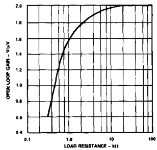
Open Loop Gain vs. Load Resistance
