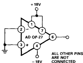
Figure 2. Burn-In Circuit
