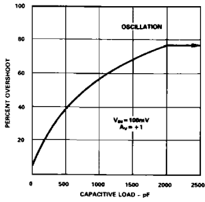
Small Signal Overshoot vs. Capacitive Load
