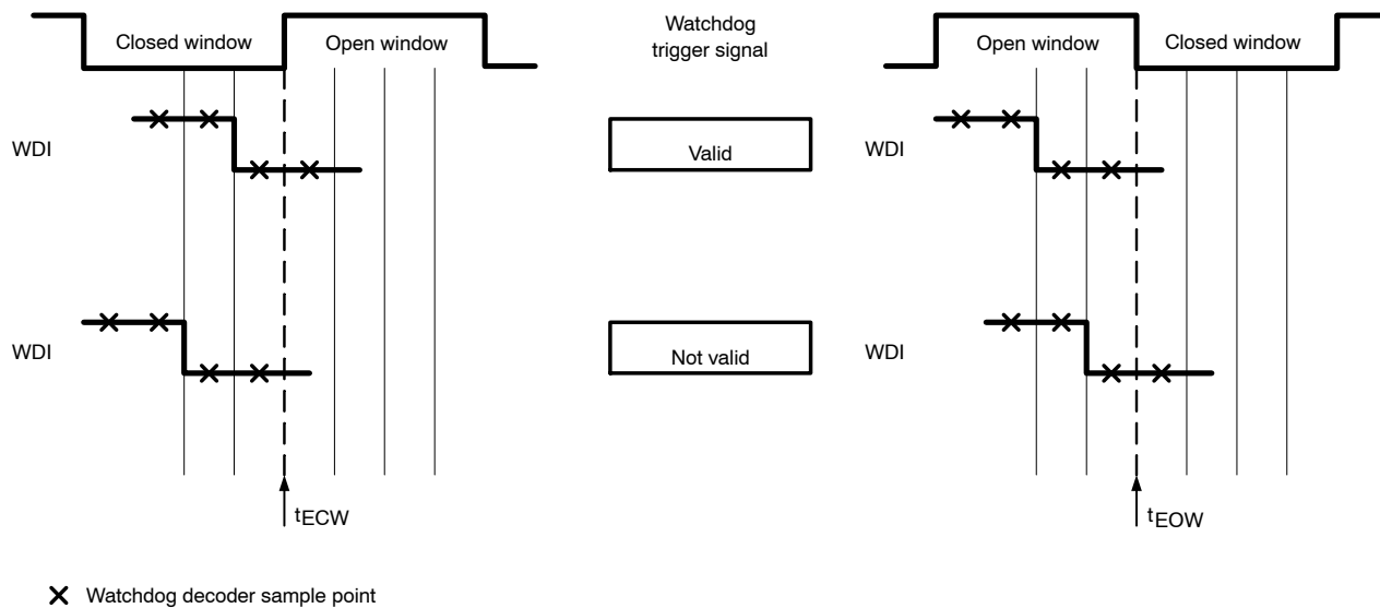
Figure 27. Valid WDI trigger signal
