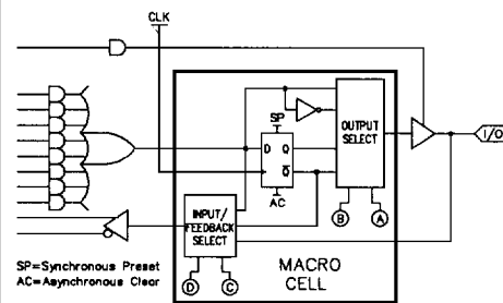
Figure 4. 22CV10Z Macro Cell Block Diagram
