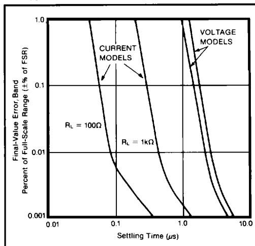
FIGURE I. Final-Value Error Band Versus Full-Scale Range Settling Time.
