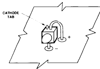
Figure 1. Proper Right Angle Mounting to a PC Board to Prevent Protruding Cathode Tab from Shorting to Anode Connection.
