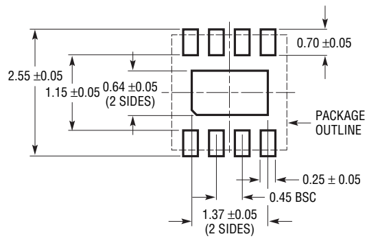
DC Package 8-Lead Plastic DFN (2mm × 2mm) (Reference LTC DWG # 05-08-1719 Rev A)
