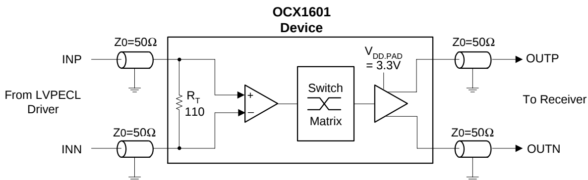
Figure 6 OCX1601 Operating in LVPECL Mode
