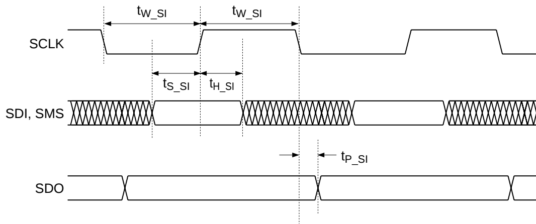
Figure 12 Serial Timing
