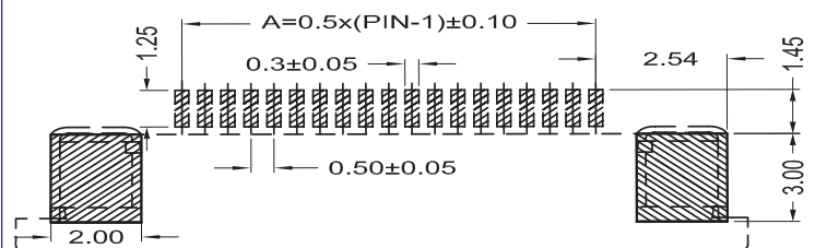
R3 and R4 PCB Layout Reference
