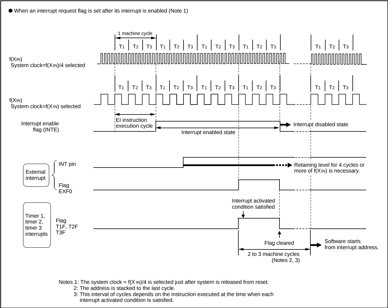
Fig. 16 Interrupt sequence
