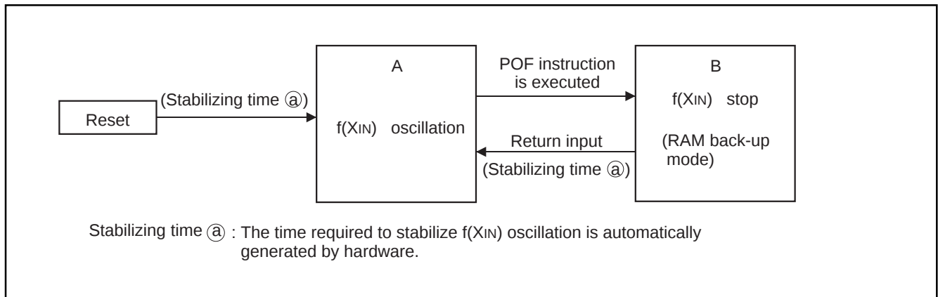
Fig. 29 State transition
