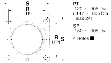
“CE” (SR) Strain Relief
