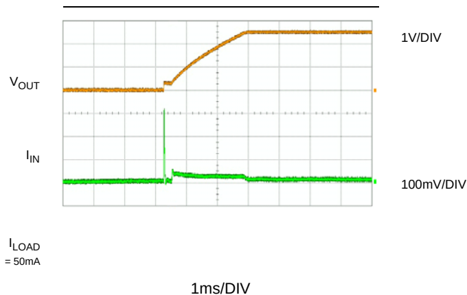
Figure 7: Rise Time with C_{OUT} = 10\mu F
