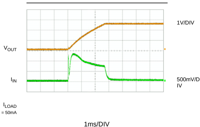
Figure 8: Rise Time with C_{OUT} = 1000\mu F
