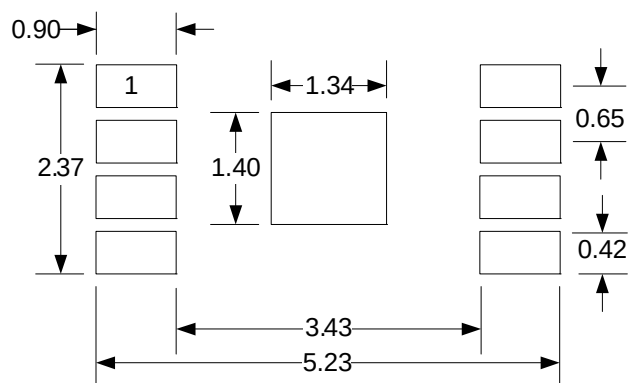
Figure 23: Recommended Solder Pad Layout for MSOP-8
