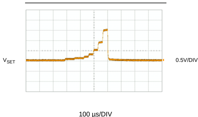
Figure 6: V_{SET} Voltage Steps for 2.5V Output
