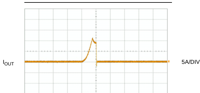
Figure 10: Current Limit Response Time
