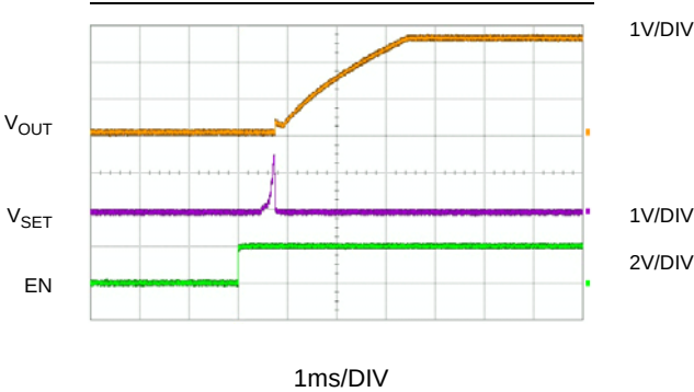
Figure 11: Startt-Up Using the Enable Pin
