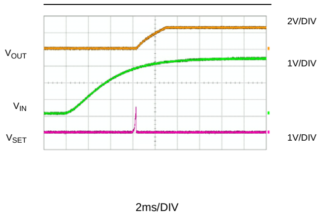
Figure 5: Startt-Up Sequence
