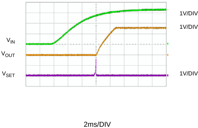
Figure 13: Input Voltage Soft Start
