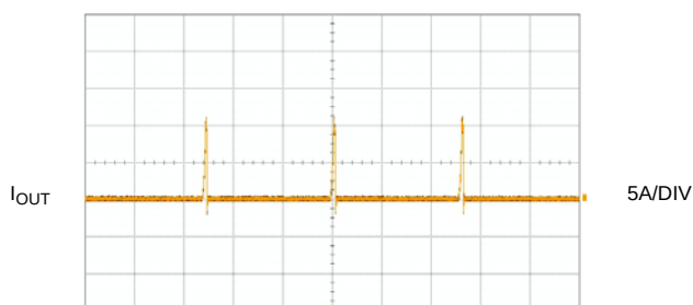
Figure 9: Hiccup Period
