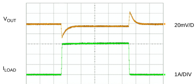
Figure 16: Load Transient Response
