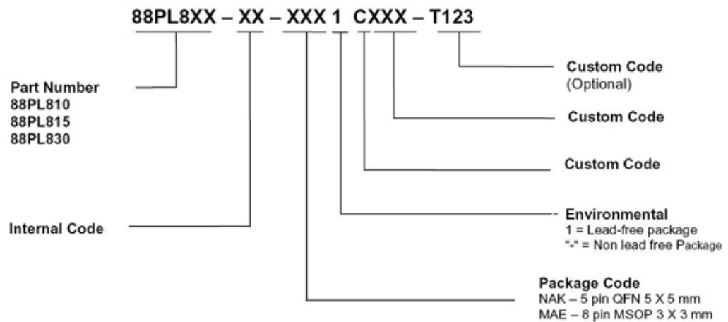
Figure 25: Ordering Part Numbers and Package Markings
