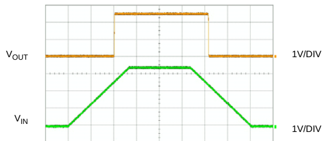
Figure 15: UVLO Thresholds
