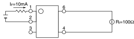
***Turn on/Turn off time measurement circuit APV1122(A)
