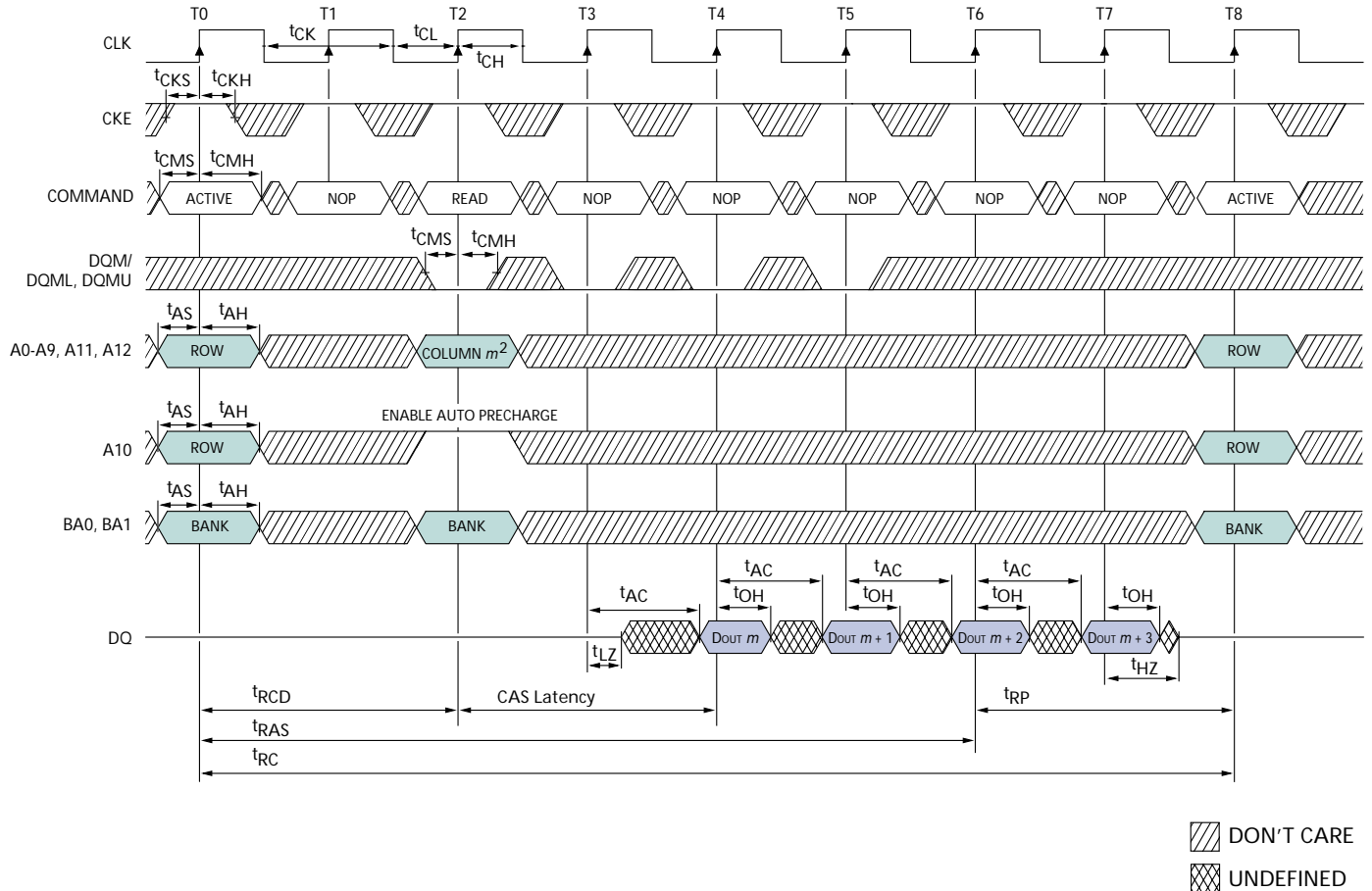
Figure 40: Read – With Auto Precharge 1
