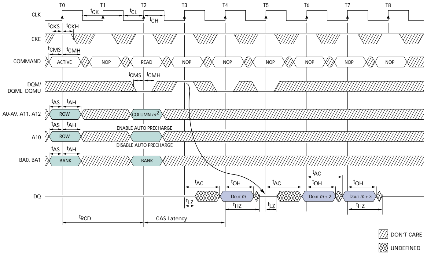
Figure 45: Read – DQM Operation 1
