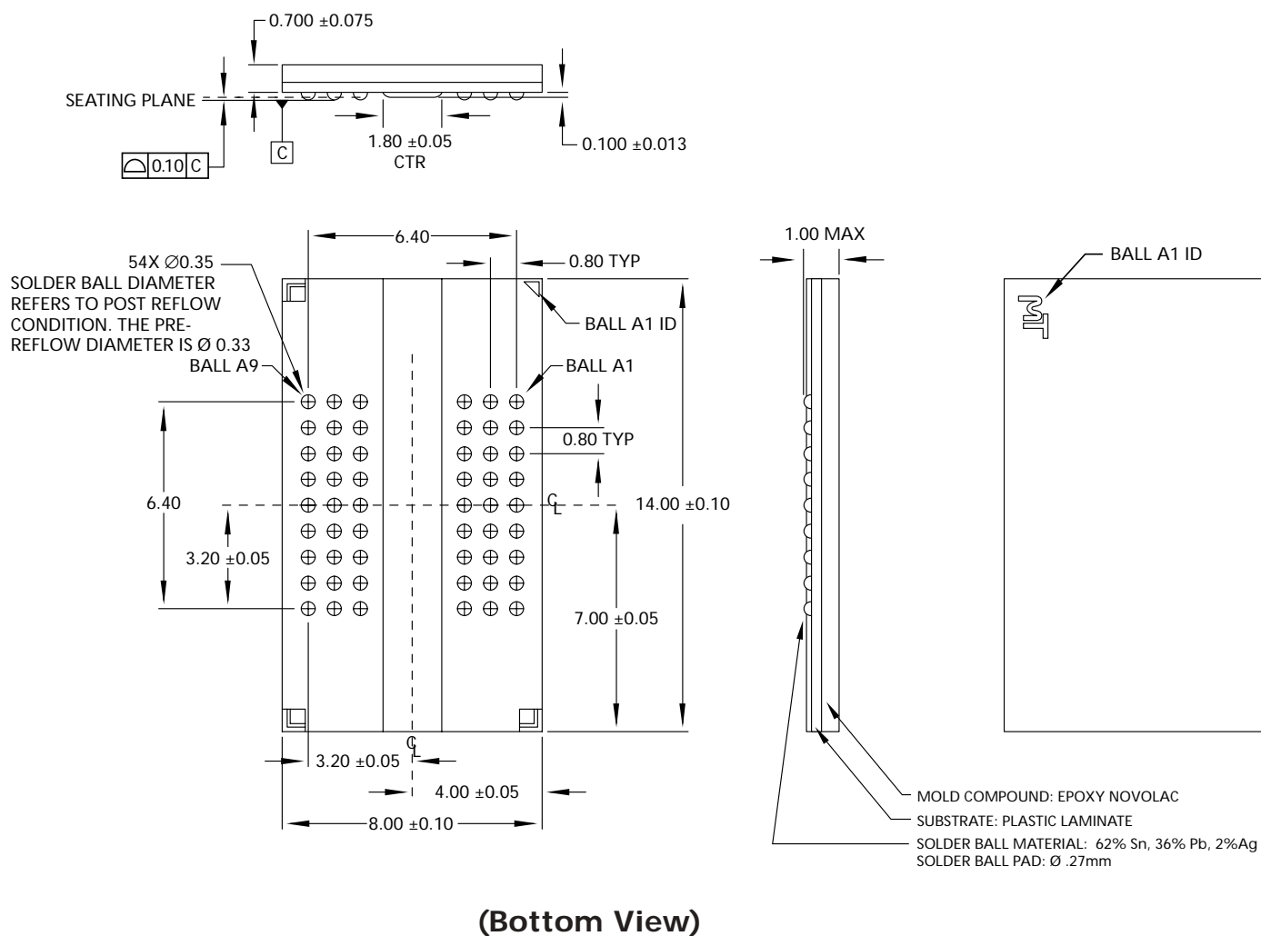
Figure 55: FBGA "FG" Package, 54-ball, 8mm x 14mm x16
