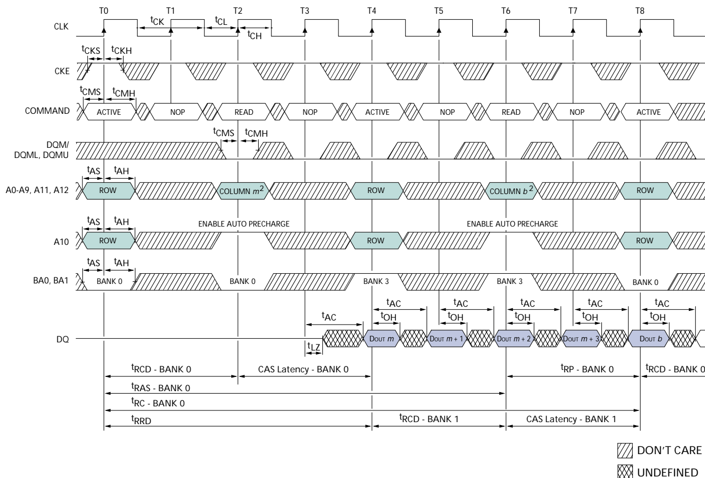
Figure 43: Alternating Bank Read Accesses 1
