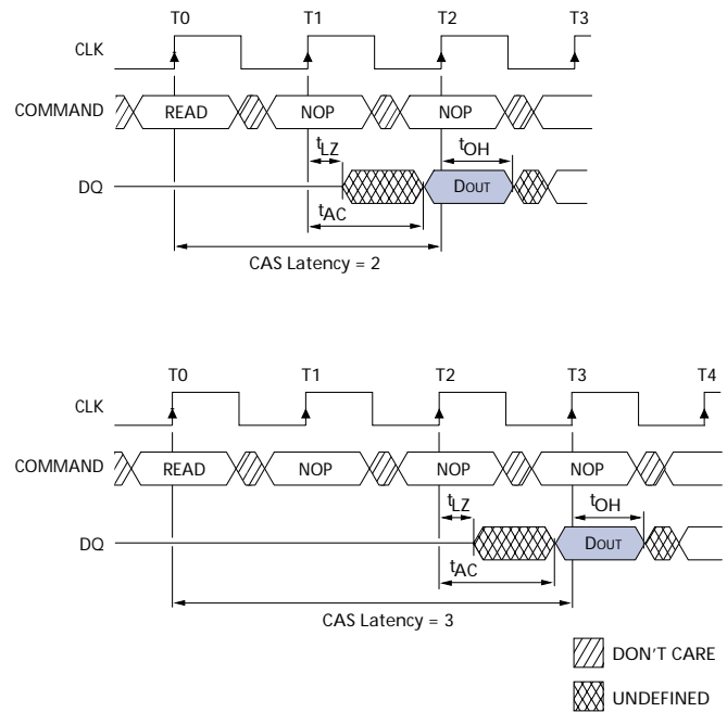
Figure 12: CAS Latency
