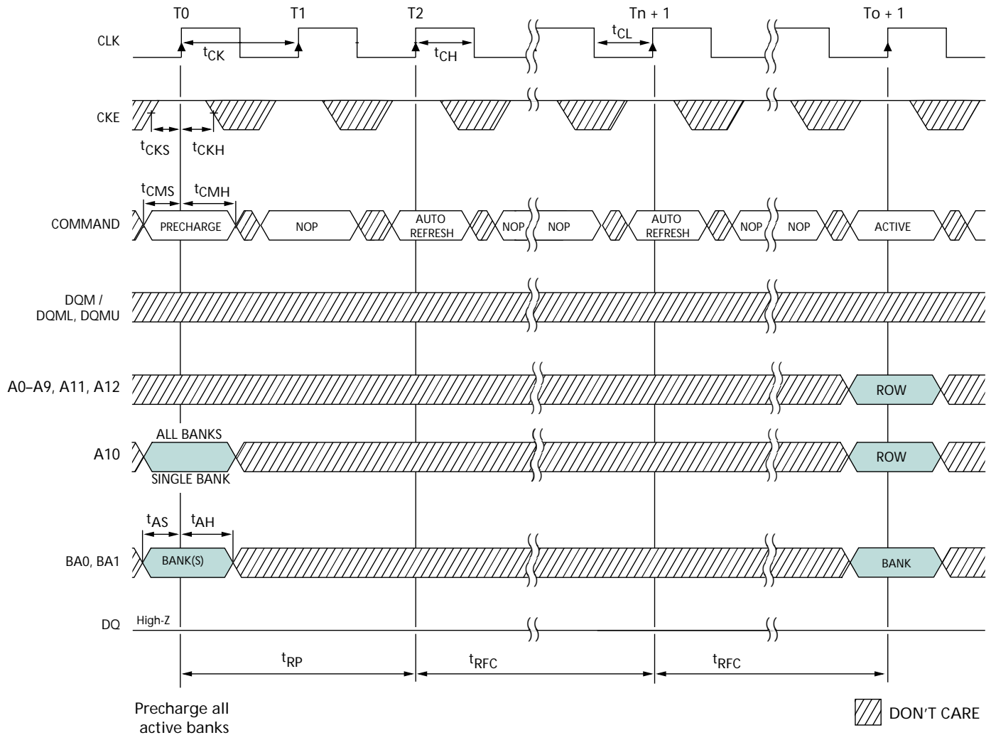
Figure 37: Auto Refresh Mode
