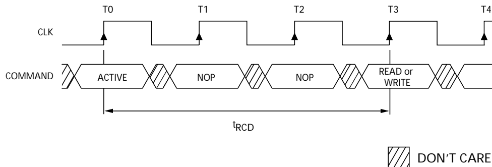
Figure 10: Example: Meeting t_{\text{RCD}} (MIN) When 2 < t_{\text{RCD}}(\text{MIN})/t_{\text{CK}} \leq 3
