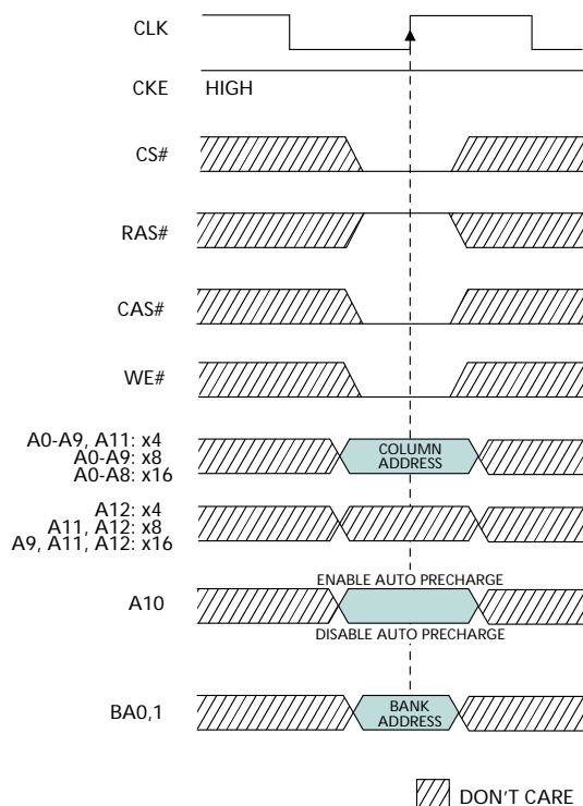
Figure 19: WRITE Command
