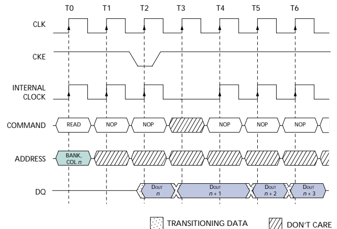
Figure 29: Clock Suspend During READ Burst
