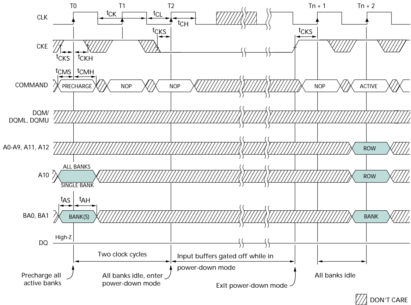
Figure35: Power-Down Mode 1
