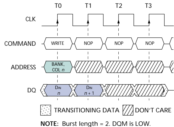
Figure 20: WRITE Burst
