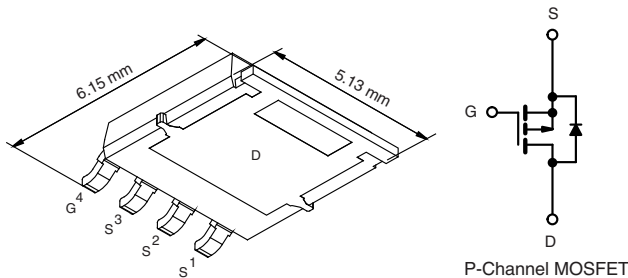
PowerPAK® SO-8L Single
