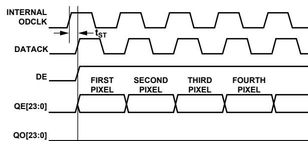
Figure 37. One Pixel per Clock (DATAACK Inverted)
