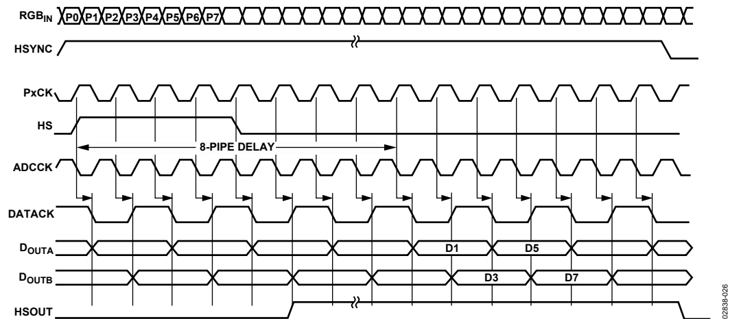
Figure 24. Dual-Channel Mode, Interleaved Outputs, Alternate Pixel Sampling (Odd Pixels, Analog Interface), Outphase = 0
