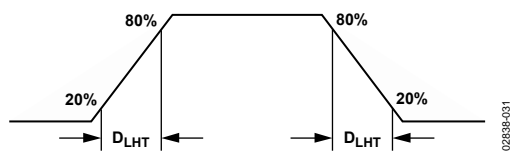
Figure 33. Digital Output Rise and Fall Times
