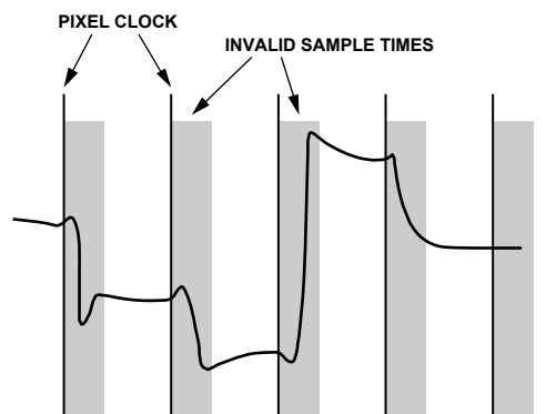
Figure 9. Pixel Sampling Times
