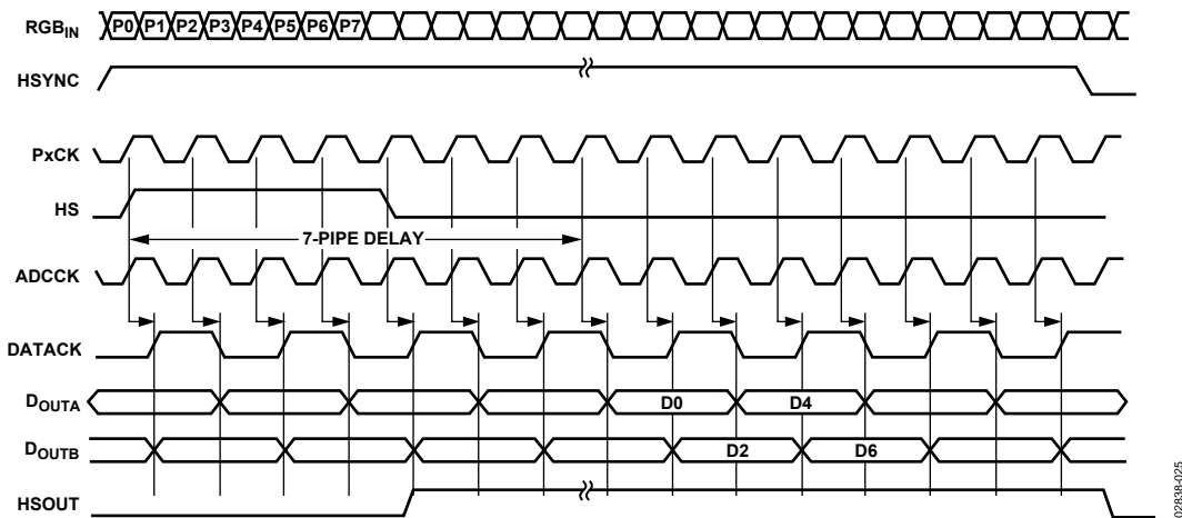
Figure 23. Dual-Channel Mode, Interleaved Outputs, Alternate Pixel Sampling (Even Pixels, Analog Interface), Outphase = 0
