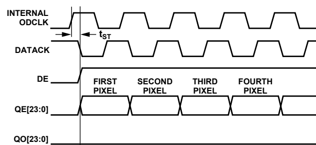
Figure 38. One Pixel per Clock (DATAACK not Inverted)
