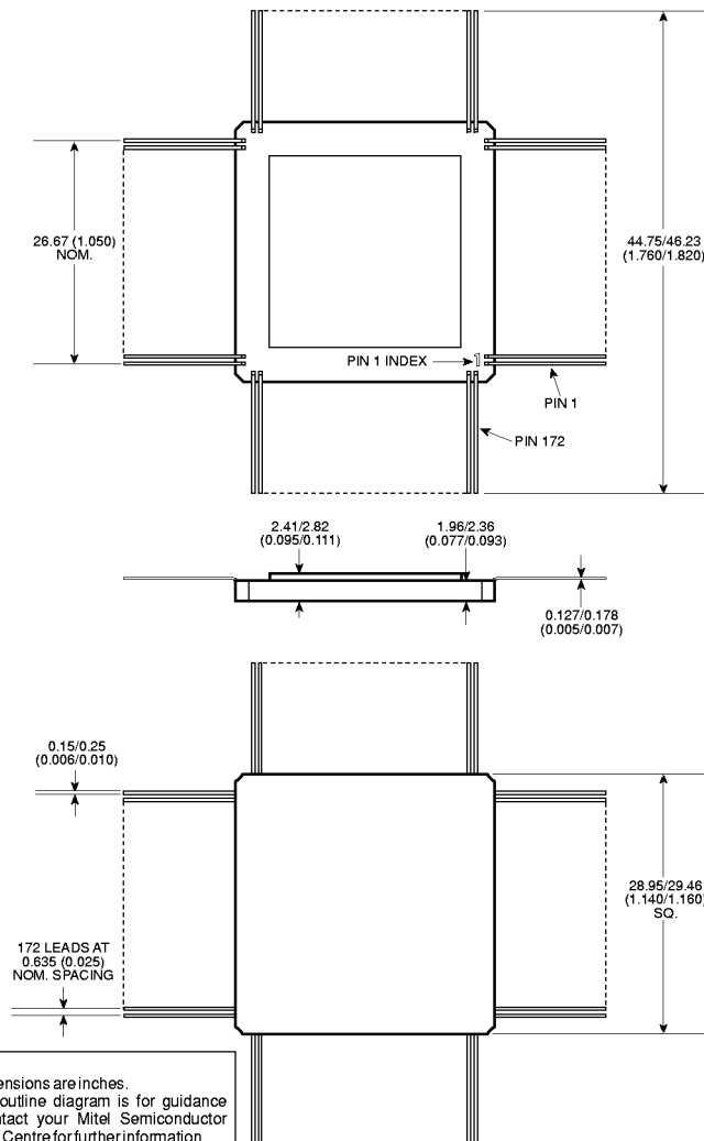
172-LEAD CERAMIC FLATPACK - GC172
