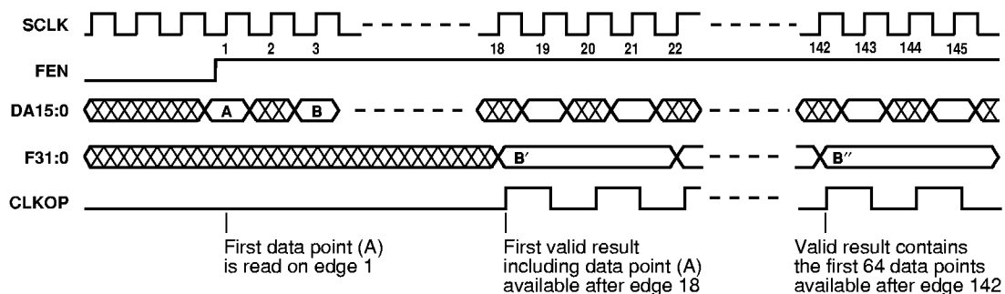
Fig. 7 Single Filter timing diagrams
