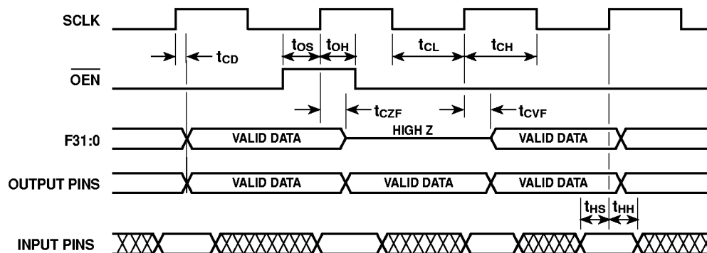
Fig. 22 Operating timings
