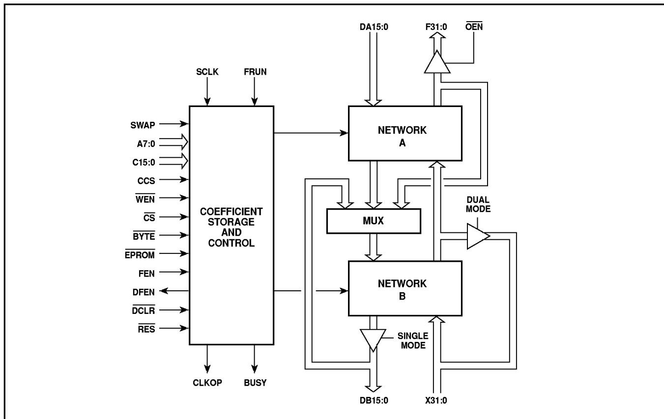
Fig. 4 Block Diagram
