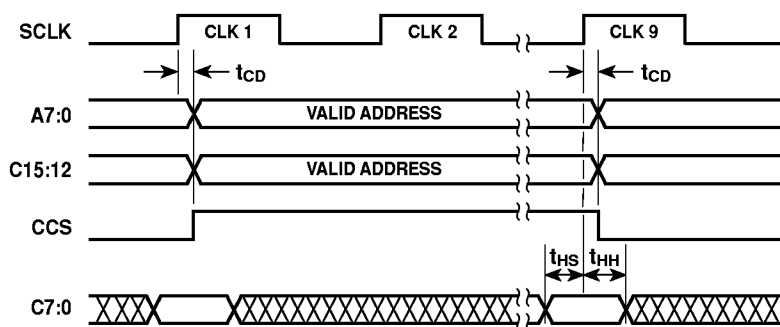
Fig. 21 EPROM load timings
