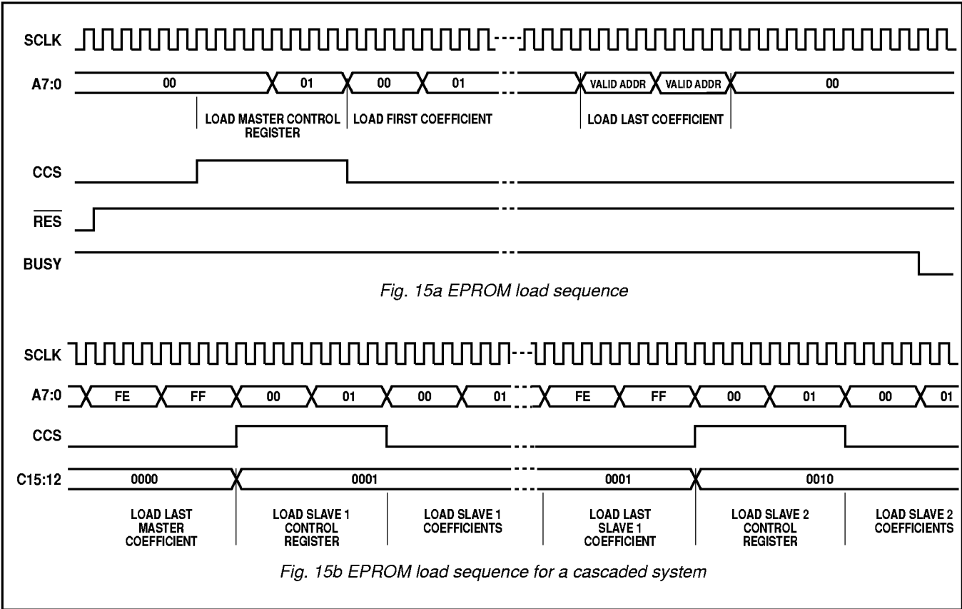
Fig. 15 EPROM load sequence timing diagrams
