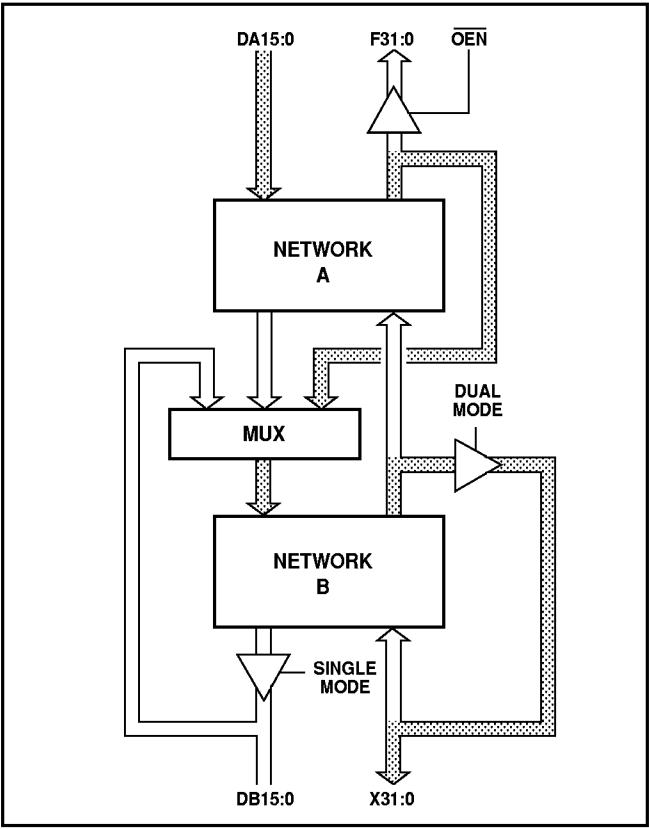
Fig. 9 Dual cascaded filter bus utilisation
