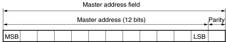
Figure 17-2. Master Address Field
