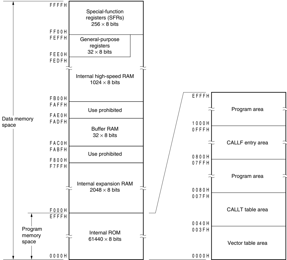
Figure 3-2. Memory Map ( \mu PD178078, 178098A)
