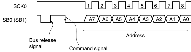
Figure 13-15. Addresses
