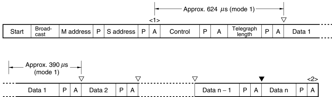
Figure 17-29. Master Transmission
