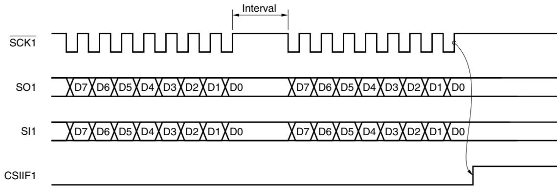
Figure 14-24. Interval Time of Automatic Transmission/Reception
