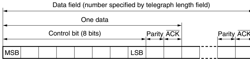
Figure 17-6. Data Field
