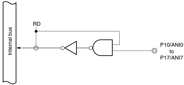
Figure 4-3. Block Diagram of P10 to P17
