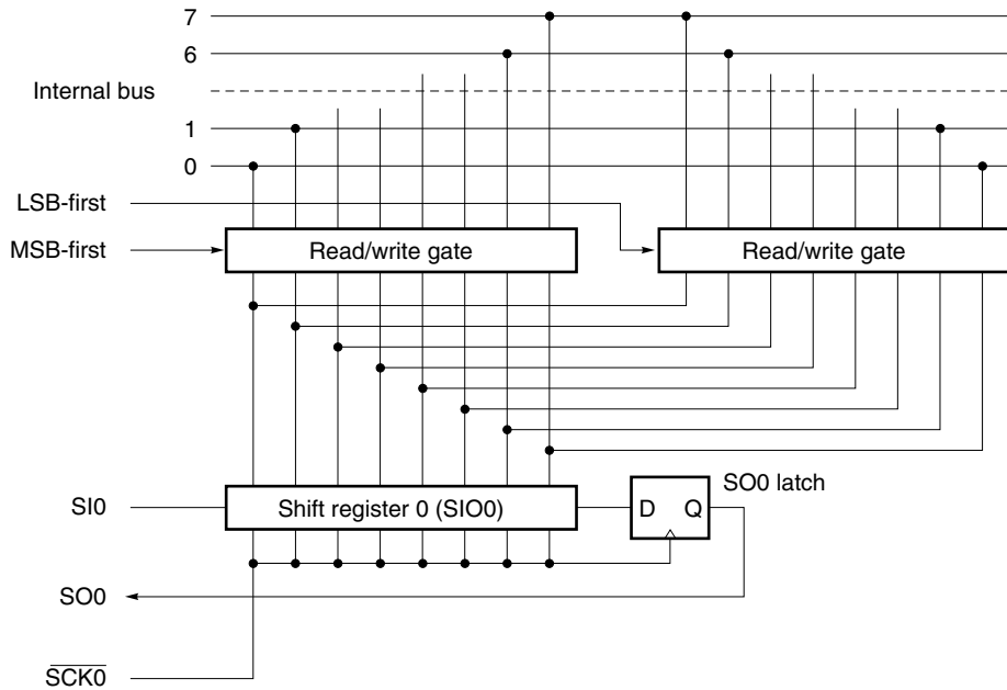
Figure 13-10. Circuit for Switching Transfer Bit Order
