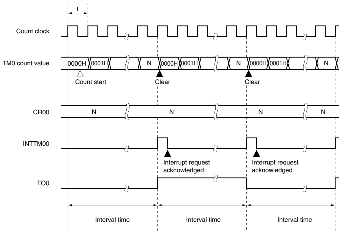
Figure 6-9. Timing of Interval Timer Operation
