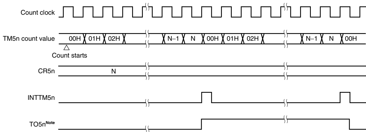
Figure 7-10. Timing of Square-Wave Output Operation
