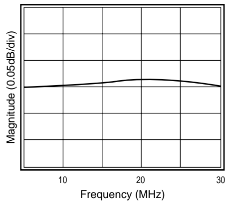
Gain Flatness
