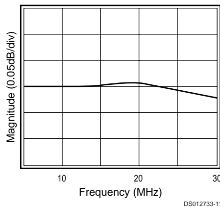
Gain Flatness
