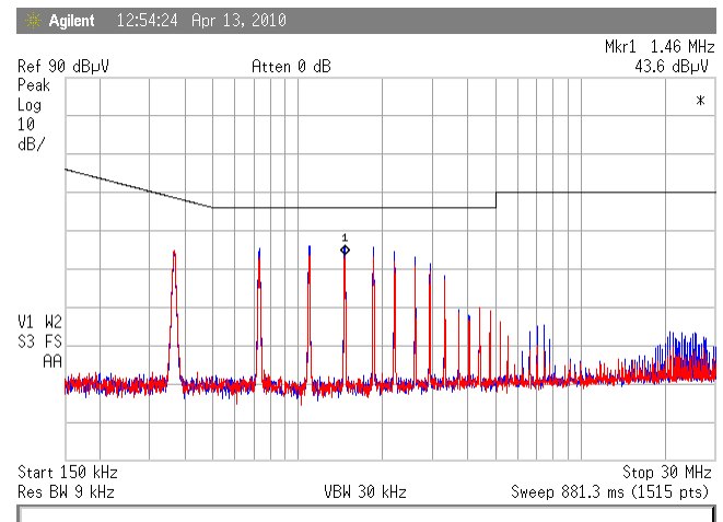
Figure 9 – V24B12C200BN using base-plate “Y” capacitors with a 136W load.
