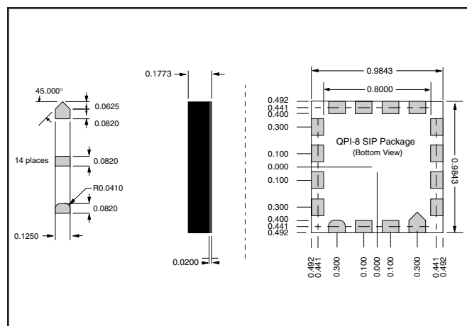
Figure 14 – LGA Pad, package height and pad location dimensions in inches.
