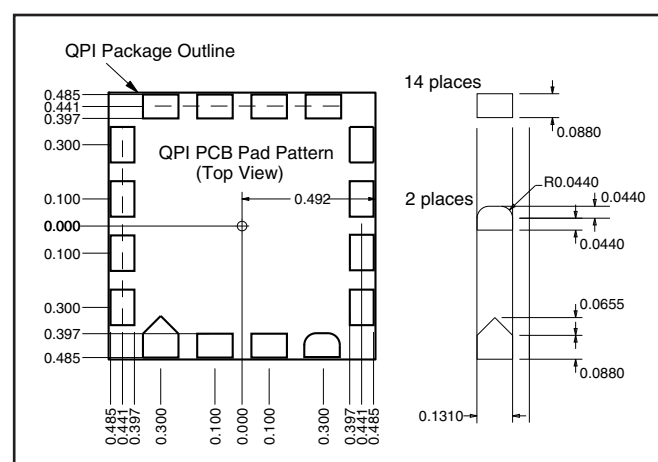
Figure 16 – Recommended PCB receiving footprint.
