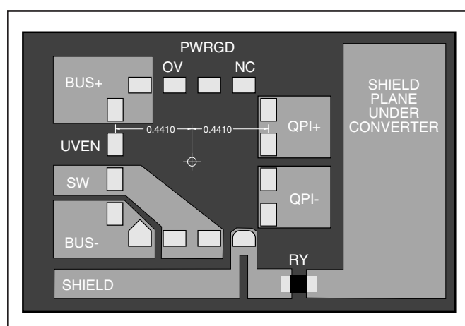
Figure 15 – Recommended PCB layout pattern.
