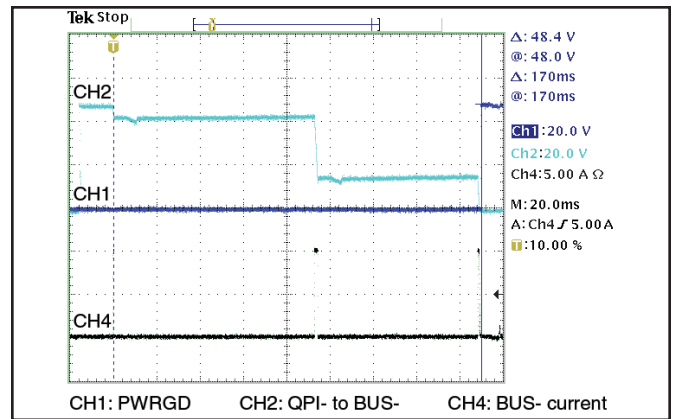
Figure 10 – 470 \mu F capacitor @ 48 V
