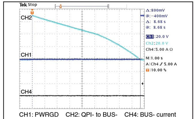
Figure 11 – 4700 \mu F capacitor @ 72 V
