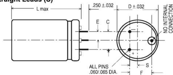
Straight Leads (S)
