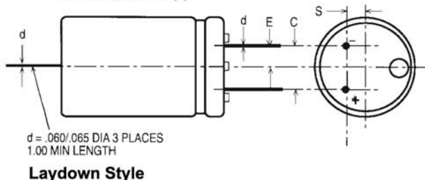
LAY DOWN, 3 LEADS (L)
