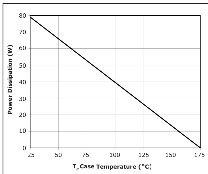
Figure 6. Power Derating
