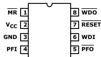
IS-705RH (8 LD FLATPACK) TOP VIEW
