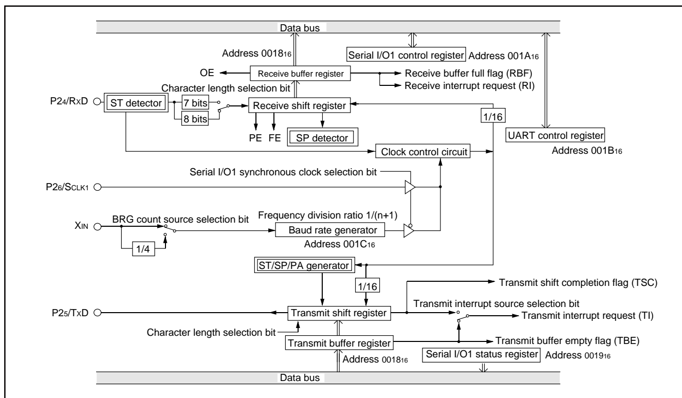
Fig. 19 Block diagram of UART serial I/O1
