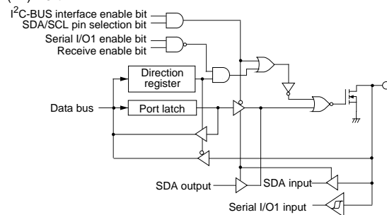
(14) Port P24
