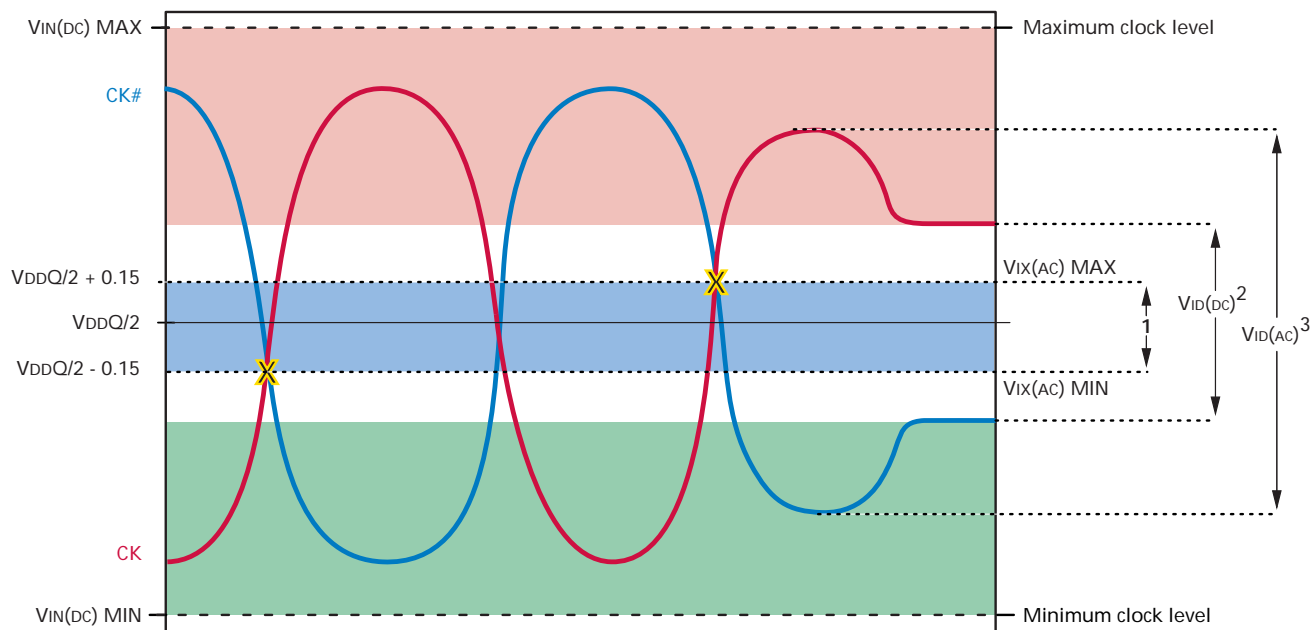
Figure 9: Clock Input
