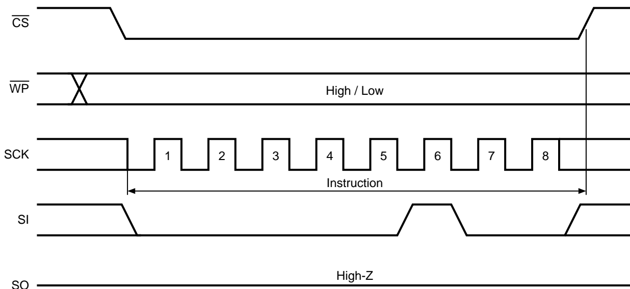
Figure 11 WRDI Operation
