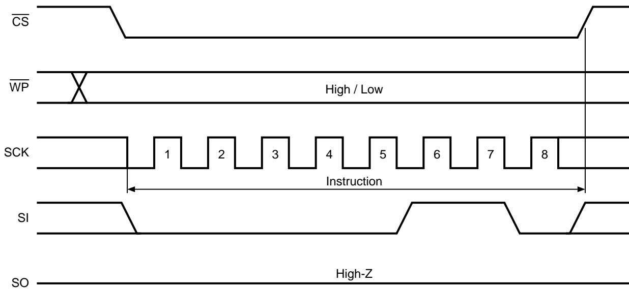
Figure 10 WREN Operation
