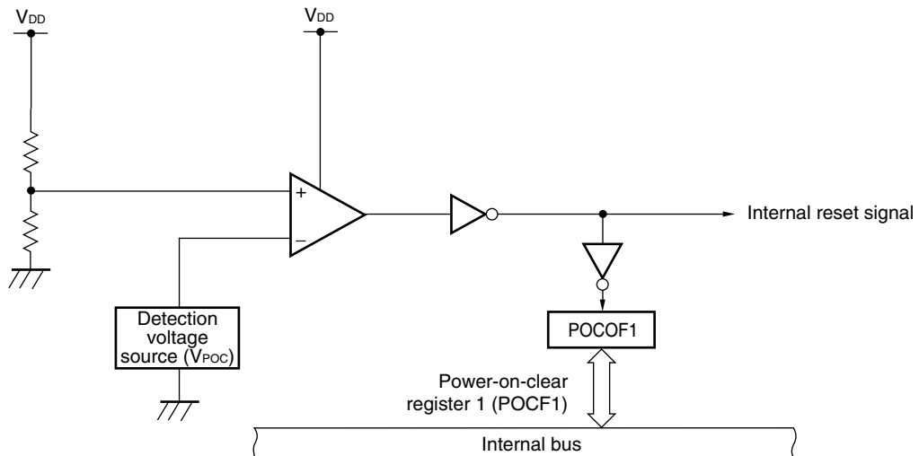
Figure 11-1. Block Diagram of Power-on-Clear Circuit
