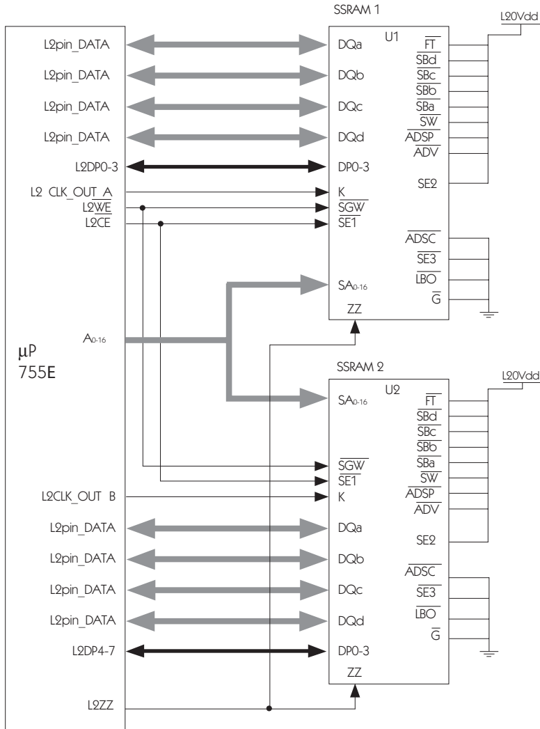
FIG. 3 BLOCK DIAGRAM, L2 INTERCONNECT
