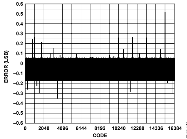
Figure 19. AD9736 DNL, 25°C, 20 mA FS
