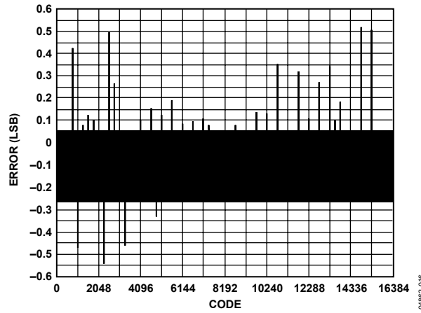
Figure 18. AD9736 DNL, -40°C, 20 mA FS
