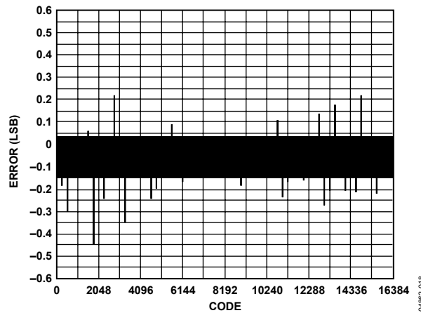
Figure 20. AD9736 DNL, 85°C, 20 mA FS
