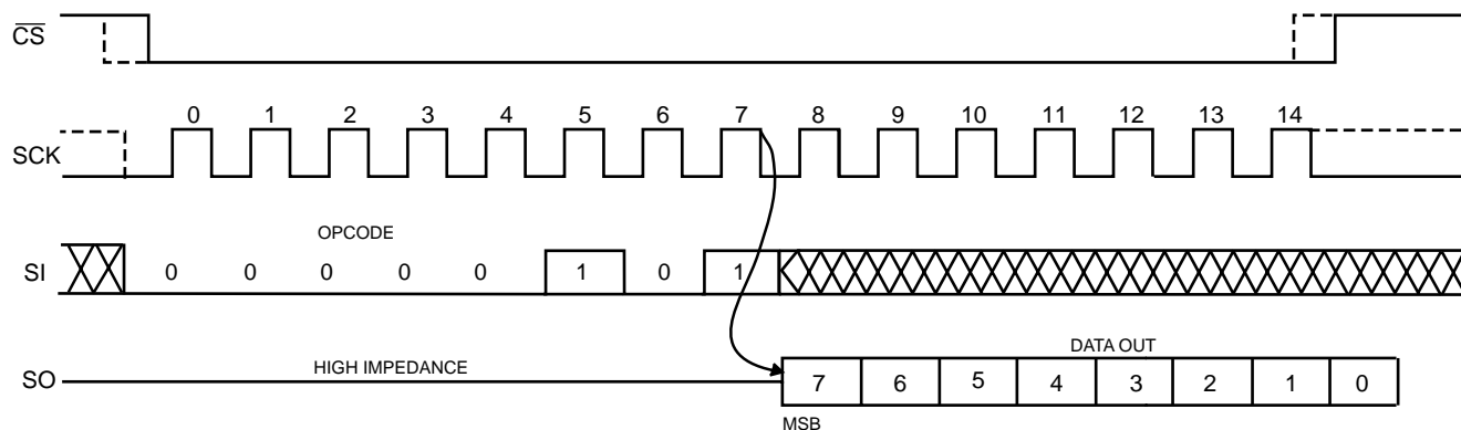
Figure 5. RDSR Timing
