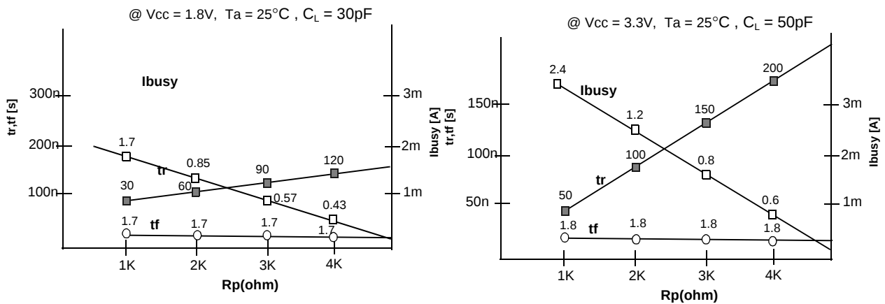
Figure 17. R_p vs t_r, t_f & R_p vs i_{\text{busy}}
