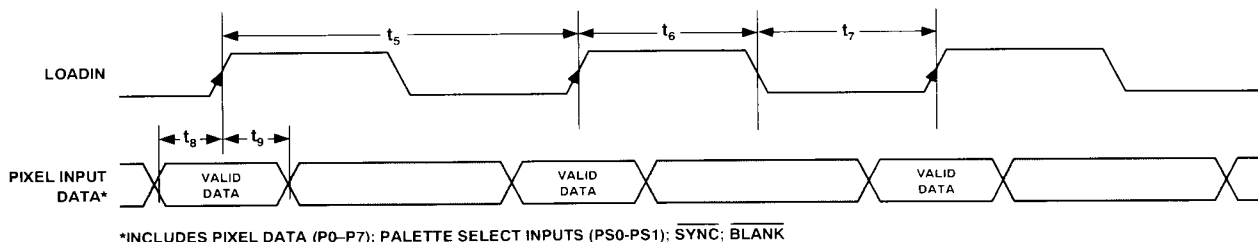
Figure 3. LOADIN vs. Pixel Input Data
