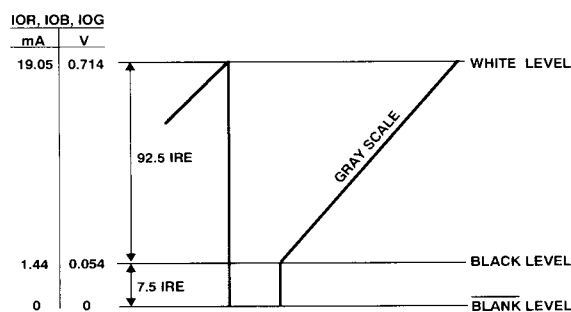
Figure 26. Composite Video Waveform; Pedestal = 7.5 IRE; R_{SET} = 280 \Omega
