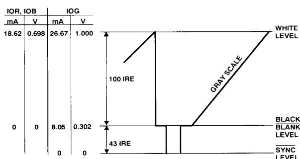
Figure 25. Composite Video Waveform \overline{\text{SYNC}} Decoded on IOG; Pedestal = 0 IRE; R_{SET} = 265 \Omega
