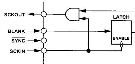
Figure 17. SCKOUT Generation Circuit
