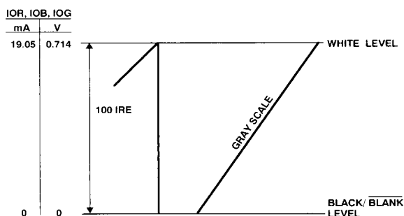
Figure 27. Composite Video Waveform; Pedestal = 0 IRE; R_{SET} = 259 \Omega
