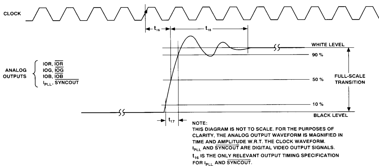
Figure 10. Analog Output Response vs. CLOCK
