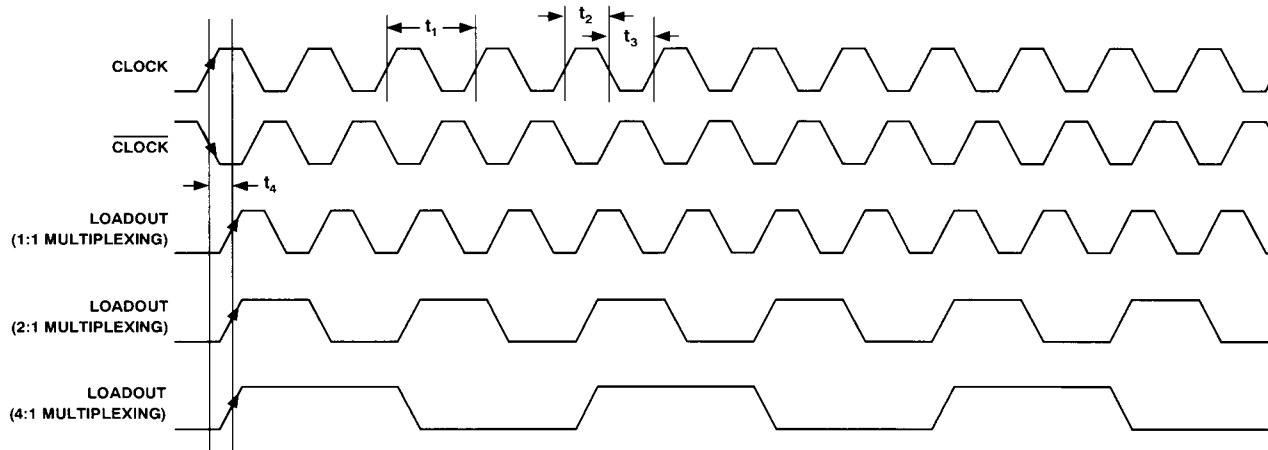
Figure 2. LOADOUT vs. Pixel Clock Input (CLOCK, \overline{\text{CLOCK}} )
