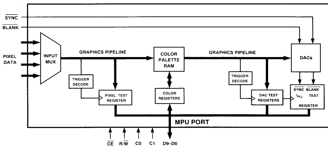
Test/Diagnostic Block Diagram
