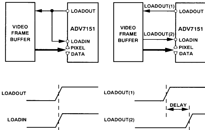
Figure 16. LOADOUT vs. Pixel Clock Input (CLOCK, CLOCK)
