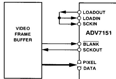
Figure 18. ADV7151 Interface Using SCKIN and SCKOUT
