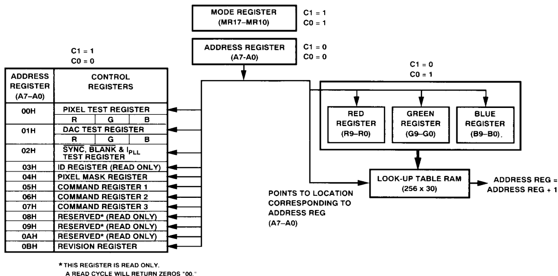
Figure 22. Internal Register Configuration and Address Decoding
