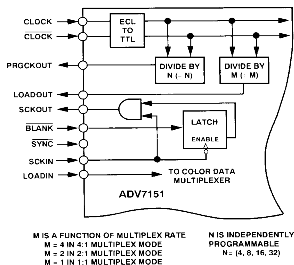
Figure 14. Clock Control Circuit of the ADV7151
