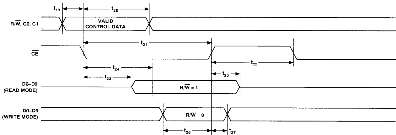
Figure 11. Microprocessor Port (MPU) Interface Timing
