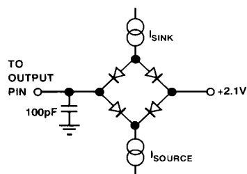
Figure 1. Load Circuit for Databus Access and Relinquish Times
