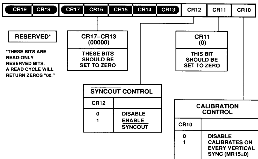
Command Register 1 (CR1) (CR19-CR10)
