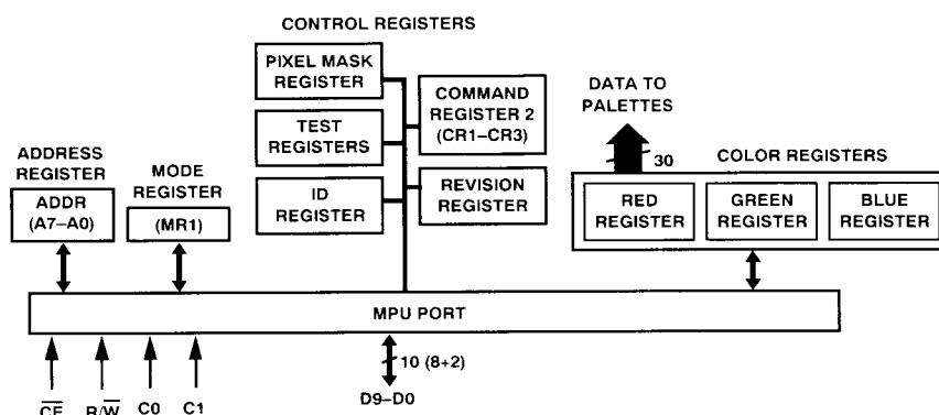
Figure 21. MPU Port and Register Configuration
