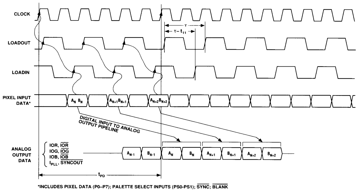
Figure 7. Pixel Input to Analog Output Pipeline with Maximum LOADOUT to LOADIN Delay (2:1 Multiplex Mode)
