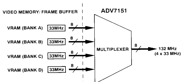
Figure 13. Direct Interfacing of Video Memory to ADV7151
