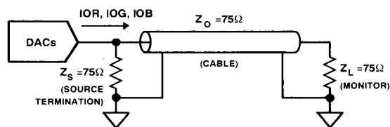
Figure 23. DAC Output Termination (Doubly Terminated 75 Ω Load)
