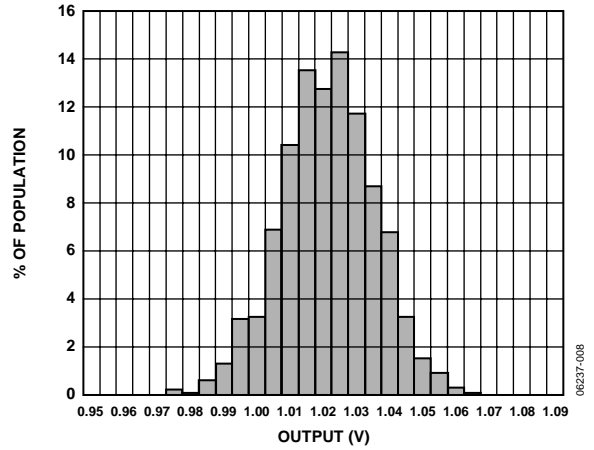
Figure 8. Y-Axis Zero g Bias at 25°C, V_s = 2V
