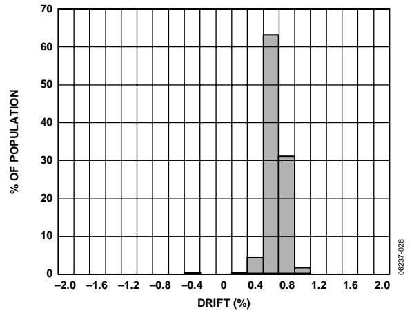
Figure 26. Y-Axis Sensitivity Drift Over Temperature, V_S = 3\text{ V}
