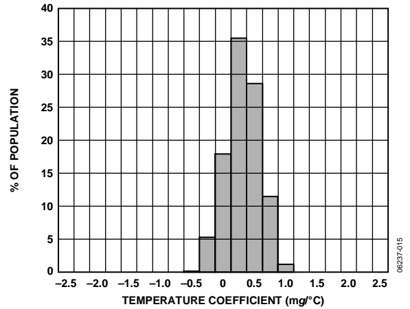
Figure 15. Y-Axis Zero g Bias Temperature Coefficient, V_s = 5 V
