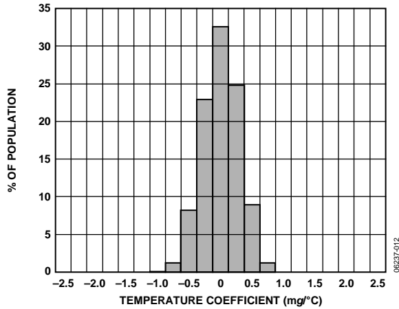
Figure 12. X-Axis Zero g Bias Temperature Coefficient, V_s = 5 V
