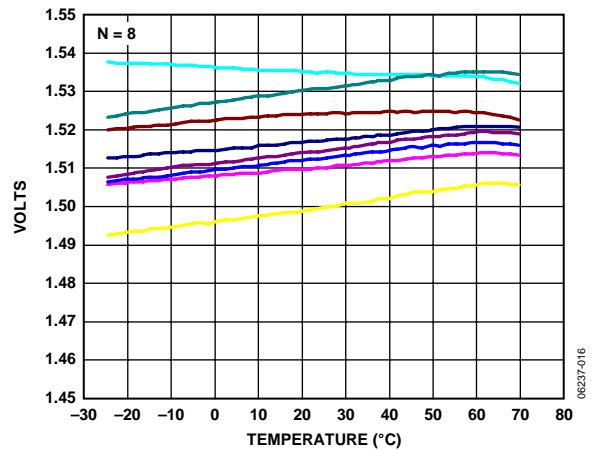
Figure 16. Y-Axis Zero g Bias vs. Temperature; Eight Parts Soldered to PCB, V_s = 3 V
