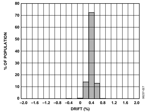
Figure 27. Y-Axis Sensitivity Drift Over Temperature, V_S = 5\text{ V}
