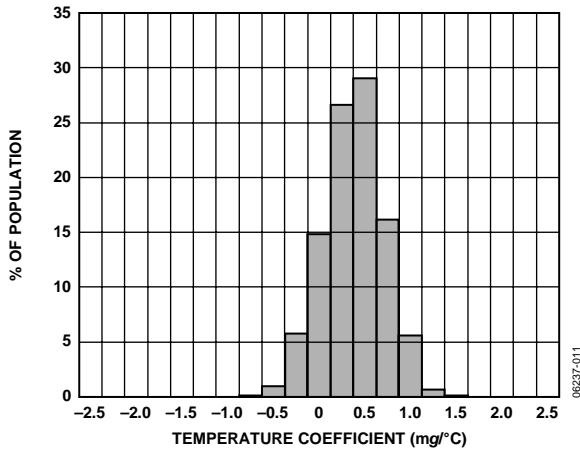
Figure 11. X-Axis Zero g Bias Temperature Coefficient, V_s = 3 V
