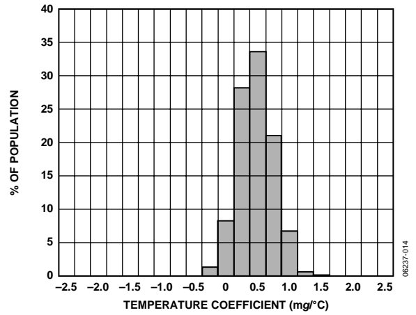
Figure 14. Y-Axis Zero g Bias Temperature Coefficient, V_s = 3 V
