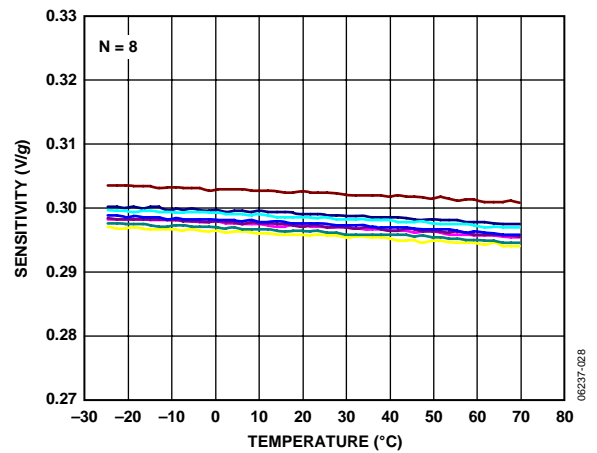
Figure 28. Y-Axis Sensitivity vs. Temperature Eight Parts Soldered to PCB, V_S = 3\text{ V}
