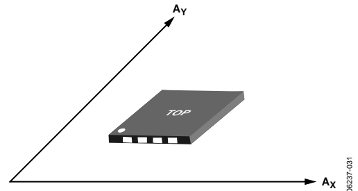
Figure 31. Axes of Acceleration Sensitivity, Corresponding Output Voltage Increases When Accelerated Along the Sensitive Axis
