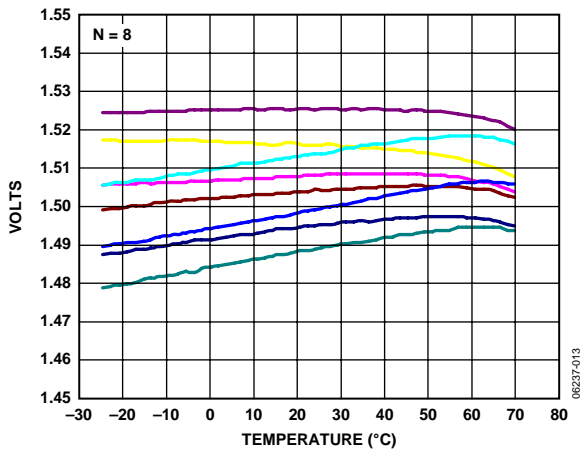
Figure 13. X-Axis Zero g Bias vs. Temperature; Eight Parts Soldered to PCB, V_s = 3 V
