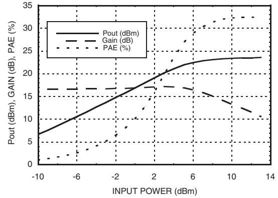
Power Compression @ 25 GHz
