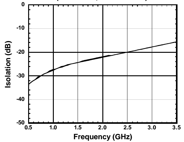
PC1-PB1 Isolation vs. Frequency
