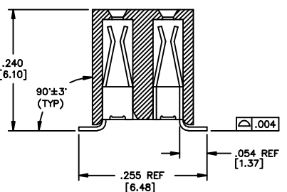
SECT "B-B"
