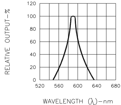
Fig.2 SPECTRAL RESPONSE
