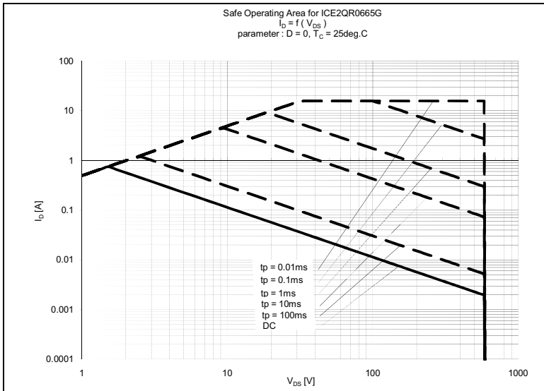
Figure 9 Safe Operating Area(SOA) curve for ICE2QR0665G
