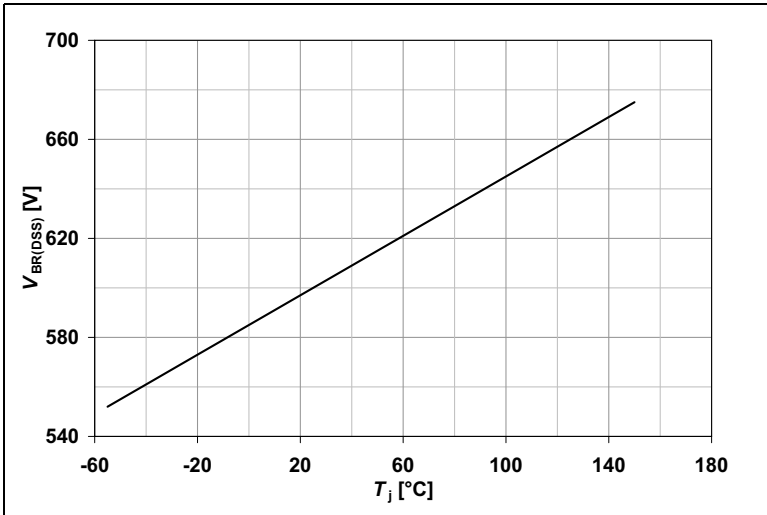
Figure 11 Drain-source breakdown voltage; V_{BR(DSS)}=f(T_j)
