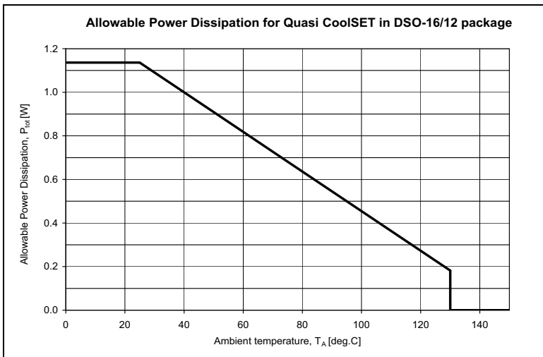
Figure 10 Power dissipation; P_{tot} = f(T_A)
