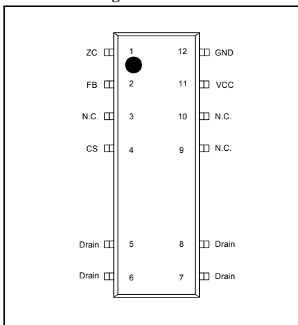
Figure 1 Pin Configuration PG-DSO-16/12 (top view)
